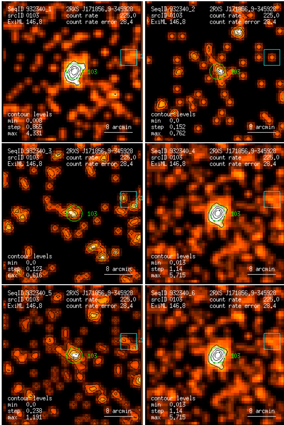
Figure 103: RASS 932340: detection 0103: band rate images, Gaussian filter: (1) PSPC channels 11 – 41, (2) 52 – 90, (3) 91 – 201, (4) 11 – 235, (5) 52 – 201, (6) 11 – 201. Broad band rates in counts/ks. Band rate contour levels in counts/ks/arcmin 2 .
