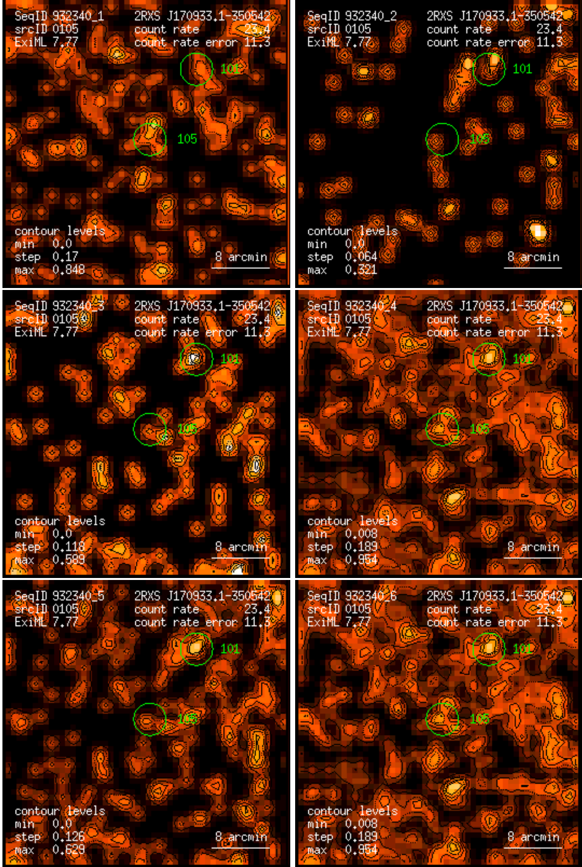
Figure 105: RASS 932340: detection 0105: band rate images, Gaussian filter: (1) PSPC channels 11 – 41, (2) 52 – 90, (3) 91 – 201, (4) 11 – 235, (5) 52 – 201, (6) 11 – 201. Broad band rates in counts/ks. Band rate contour levels in counts/ks/arcmin 2 .
