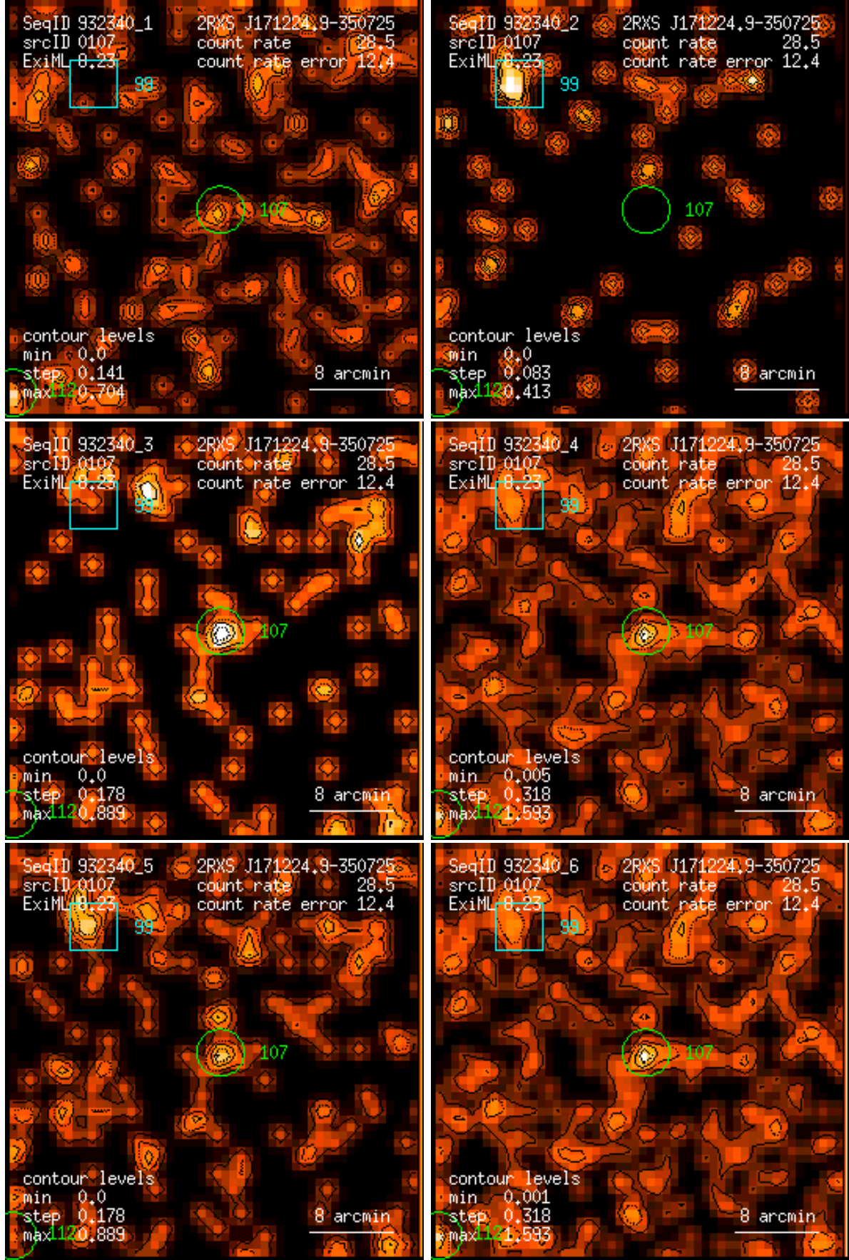
Figure 107: RASS 932340: detection 0107: band rate images, Gaussian filter: (1) PSPC channels 11 – 41, (2) 52 – 90, (3) 91 – 201, (4) 11 – 235, (5) 52 – 201, (6) 11 – 201. Broad band rates in counts/ks. Band rate contour levels in counts/ks/arcmin 2 .
