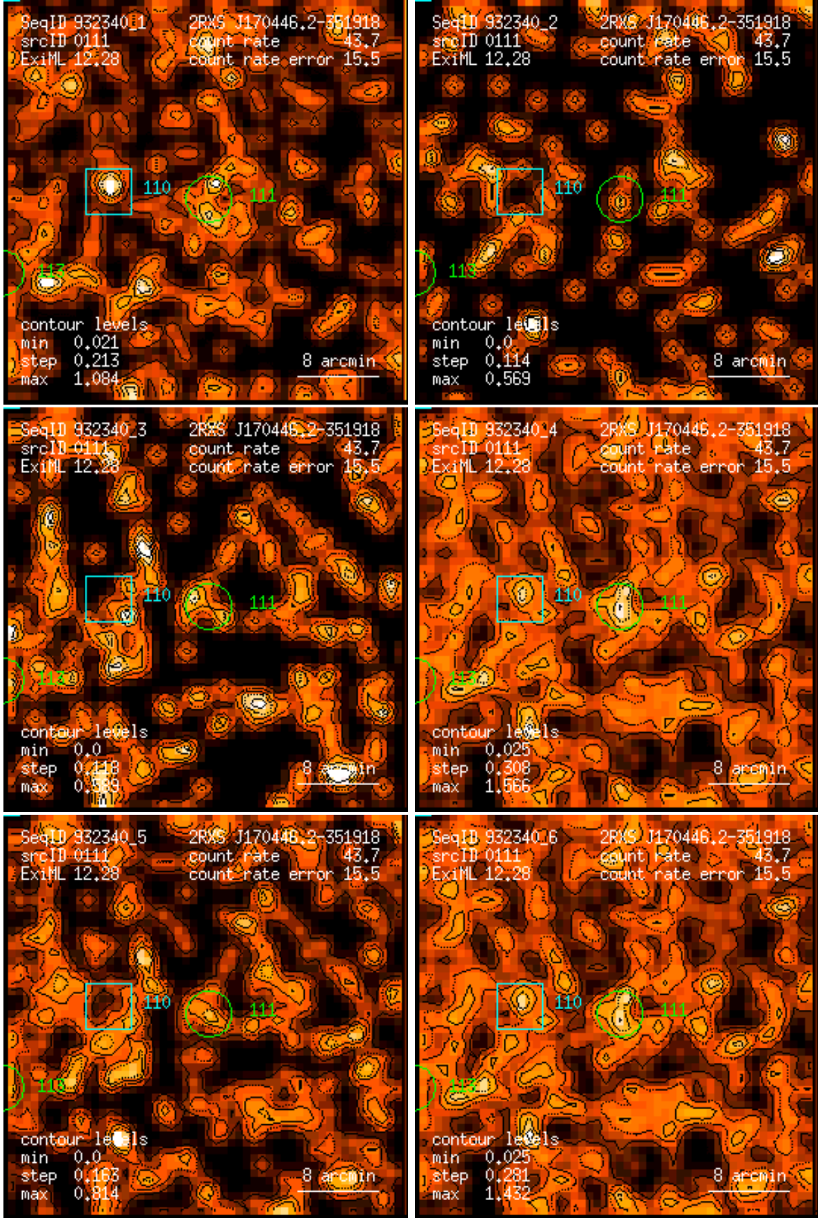
Figure 111: RASS 932340: detection 0111: band rate images, Gaussian filter: (1) PSPC channels 11 – 41, (2) 52 – 90, (3) 91 – 201, (4) 11 – 235, (5) 52 – 201, (6) 11 – 201. Broad band rates in counts/ks. Band rate contour levels in counts/ks/arcmin 2 .
