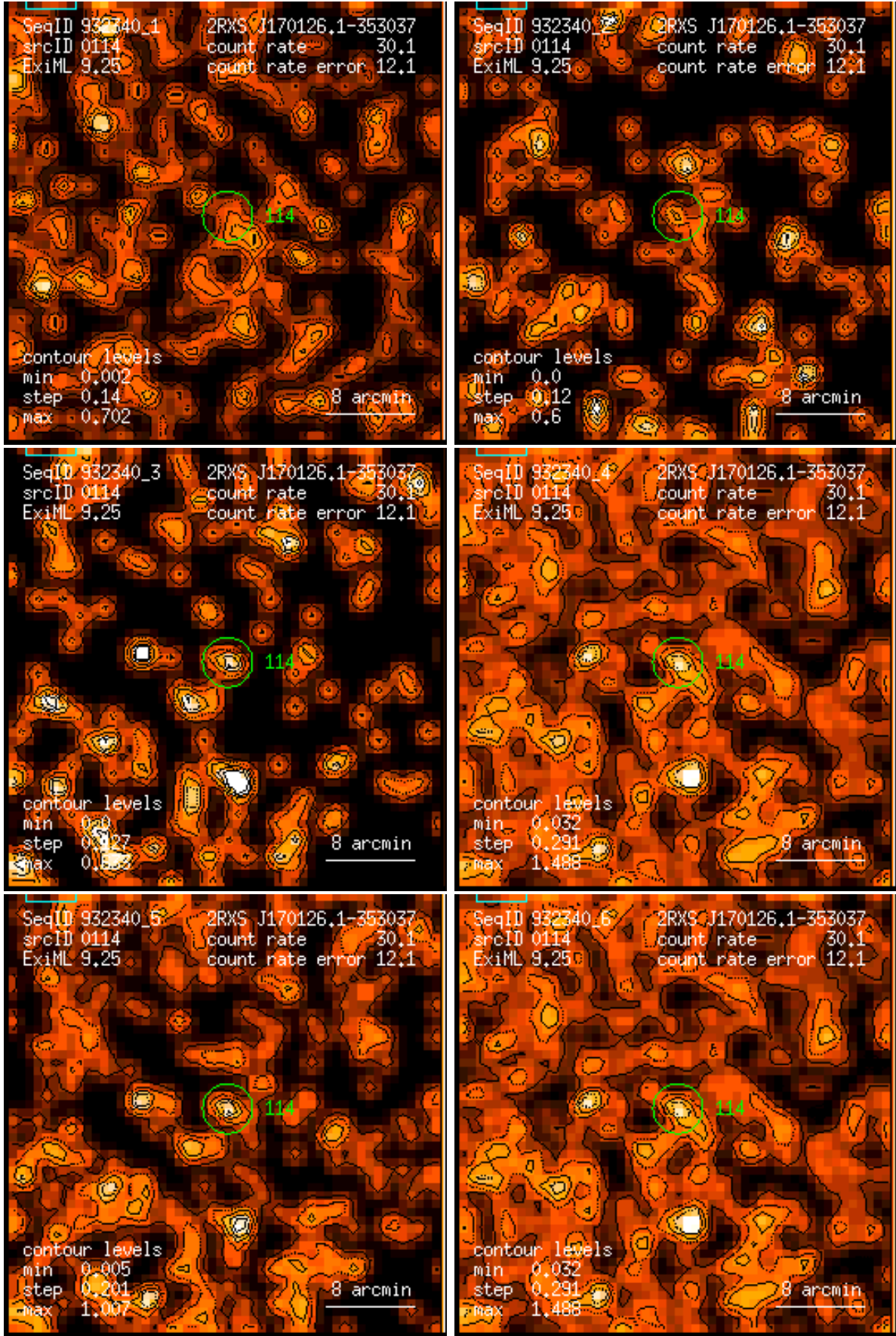
Figure 114: RASS 932340: detection 0114: band rate images, Gaussian filter: (1) PSPC channels 11 – 41, (2) 52 – 90, (3) 91 – 201, (4) 11 – 235, (5) 52 – 201, (6) 11 – 201. Broad band rates in counts/ks. Band rate contour levels in counts/ks/arcmin 2 .
