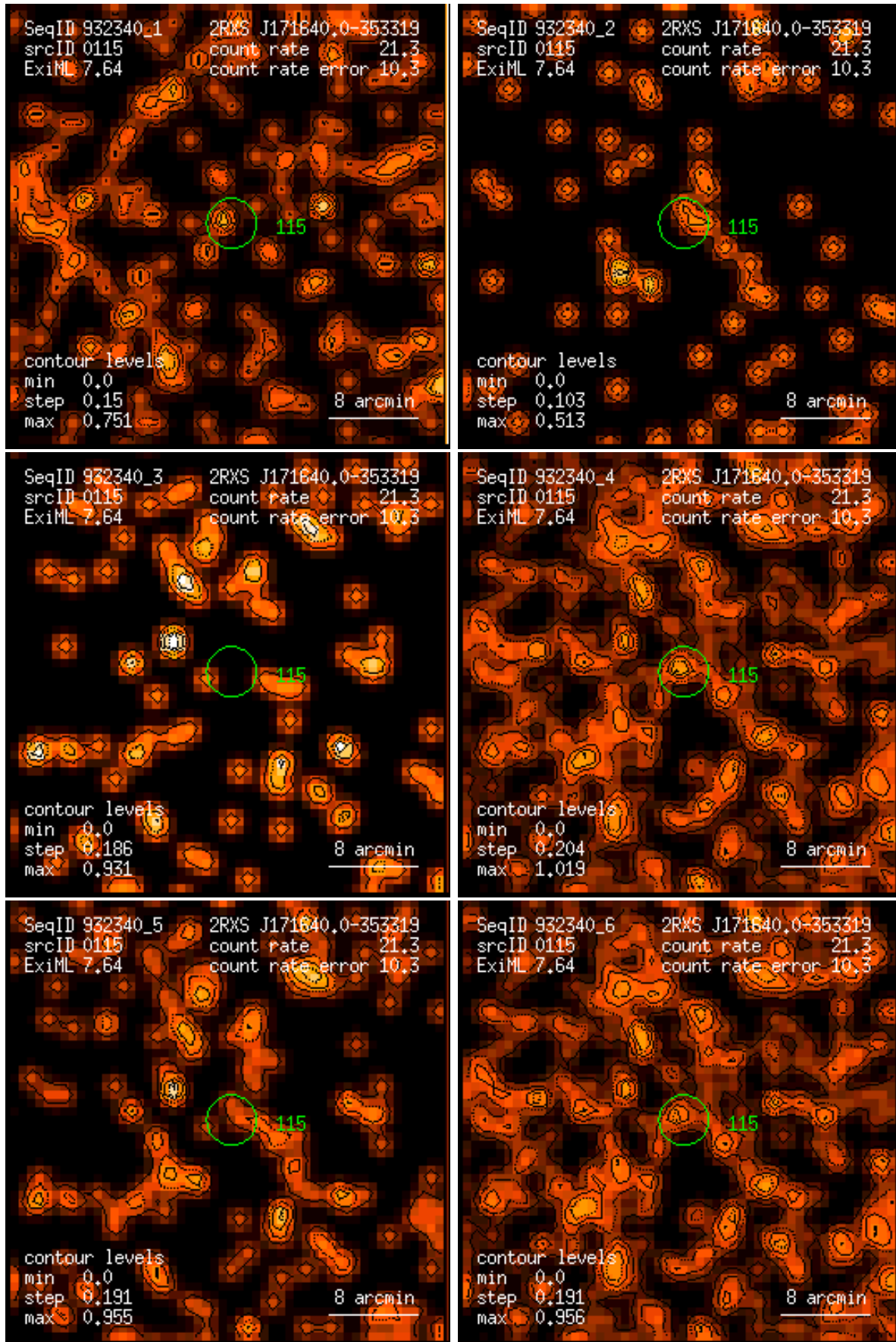
Figure 115: RASS 932340: detection 0115: band rate images, Gaussian filter: (1) PSPC channels 11 – 41, (2) 52 – 90, (3) 91 – 201, (4) 11 – 235, (5) 52 – 201, (6) 11 – 201. Broad band rates in counts/ks. Band rate contour levels in counts/ks/arcmin 2 .
