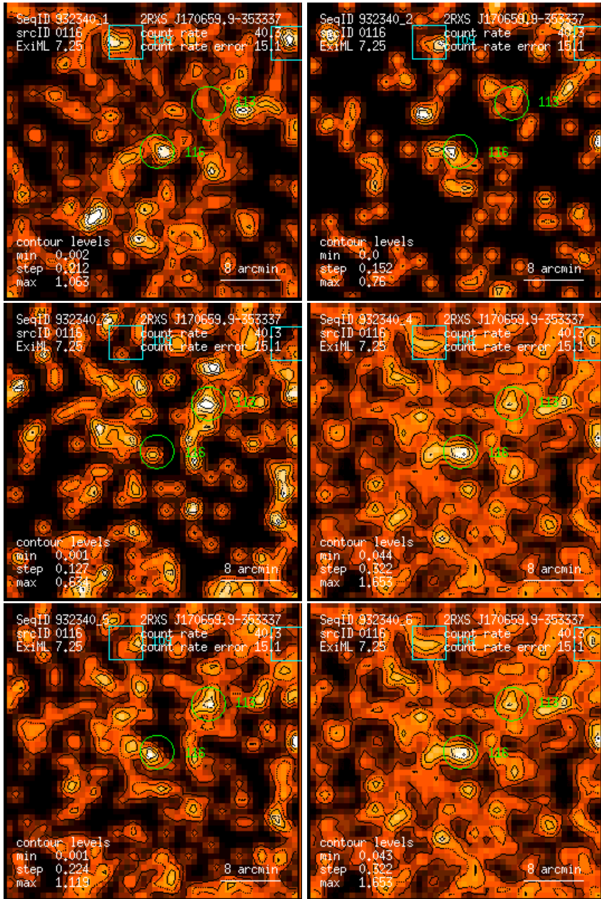
Figure 116: RASS 932340: detection 0116: band rate images, Gaussian filter: (1) PSPC channels 11 – 41, (2) 52 – 90, (3) 91 – 201, (4) 11 – 235, (5) 52 – 201, (6) 11 – 201. Broad band rates in counts/ks. Band rate contour levels in counts/ks/arcmin 2 .
