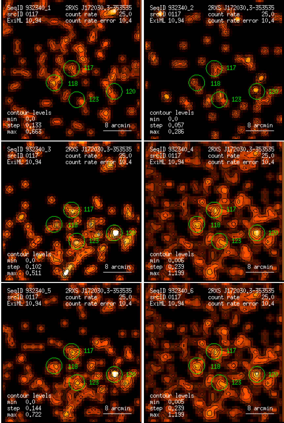
Figure 117: RASS 932340: detection 0117: band rate images, Gaussian filter: (1) PSPC channels 11 – 41, (2) 52 – 90, (3) 91 – 201, (4) 11 – 235, (5) 52 – 201, (6) 11 – 201. Broad band rates in counts/ks. Band rate contour levels in counts/ks/arcmin 2 .
