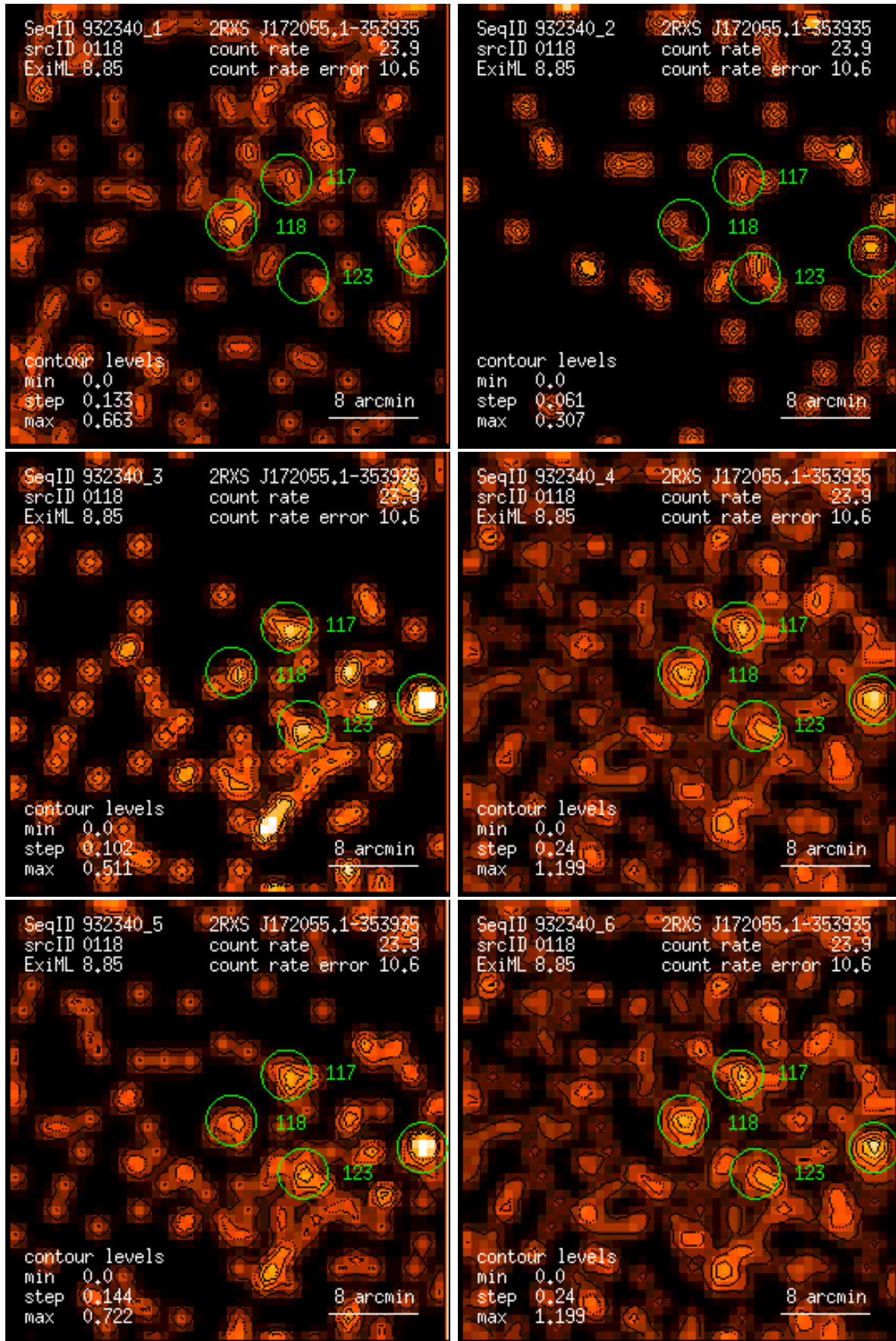
Figure 118: RASS 932340: detection 0118: band rate images, Gaussian filter: (1) PSPC channels 11 – 41, (2) 52 – 90, (3) 91 – 201, (4) 11 – 235, (5) 52 – 201, (6) 11 – 201. Broad band rates in counts/ks. Band rate contour levels in counts/ks/arcmin 2 .
