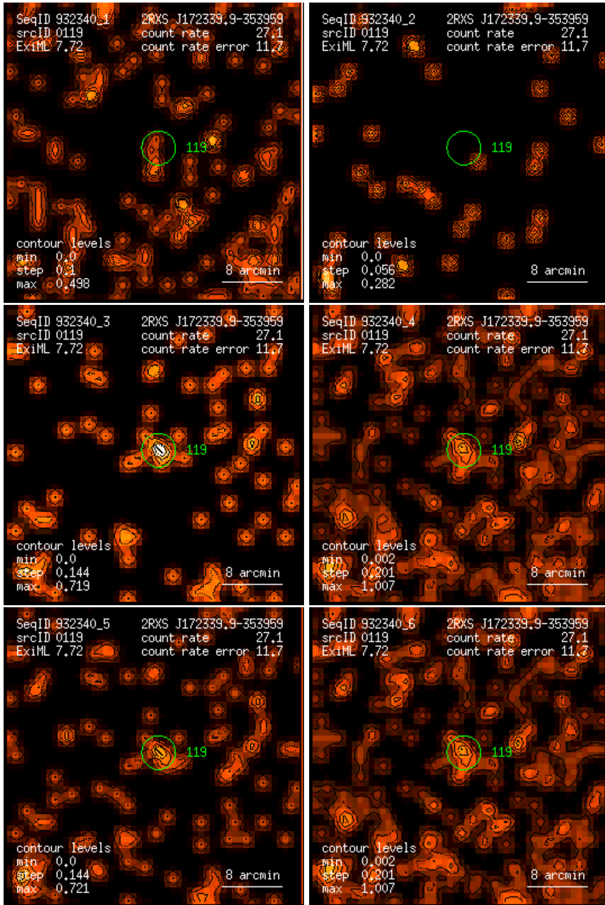
Figure 119: RASS 932340: detection 0119: band rate images, Gaussian filter: (1) PSPC channels 11 – 41, (2) 52 – 90, (3) 91 – 201, (4) 11 – 235, (5) 52 – 201, (6) 11 – 201. Broad band rates in counts/ks. Band rate contour levels in counts/ks/arcmin 2 .
