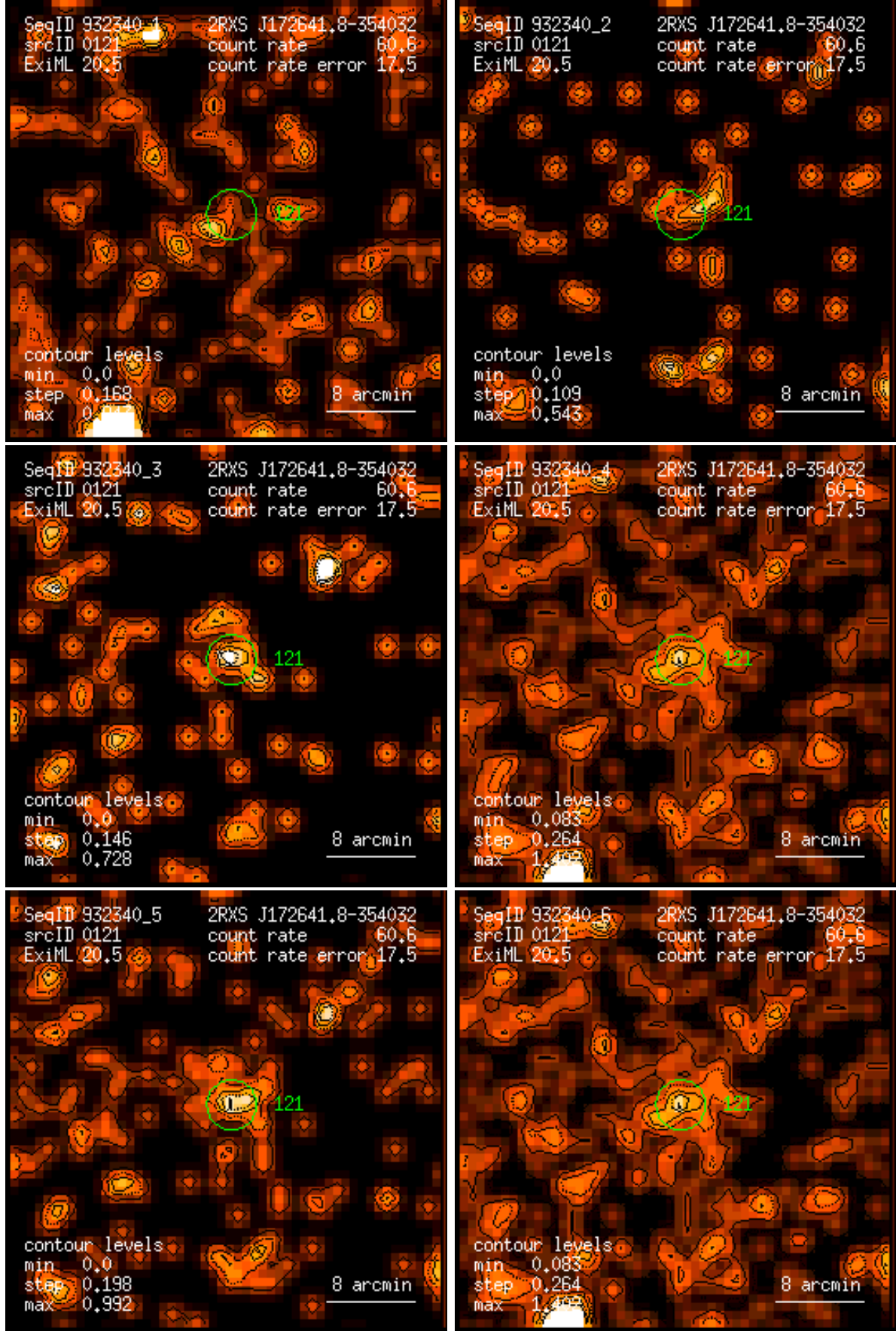
Figure 121: RASS 932340: detection 0121: band rate images, Gaussian filter: (1) PSPC channels 11 – 41, (2) 52 – 90, (3) 91 – 201, (4) 11 – 235, (5) 52 – 201, (6) 11 – 201. Broad band rates in counts/ks. Band rate contour levels in counts/ks/arcmin 2 .
