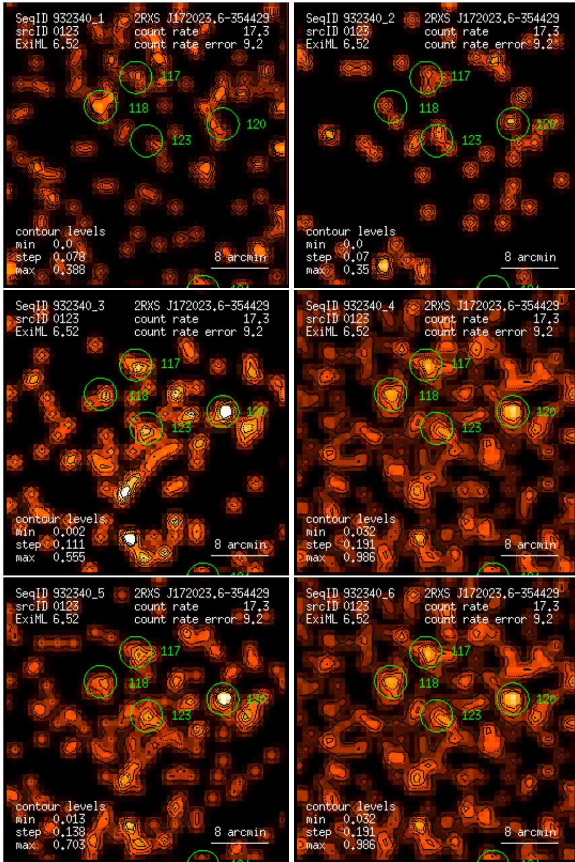
Figure 123: RASS 932340: detection 0123: band rate images, Gaussian filter: (1) PSPC channels 11 – 41, (2) 52 – 90, (3) 91 – 201, (4) 11 – 235, (5) 52 – 201, (6) 11 – 201. Broad band rates in counts/ks. Band rate contour levels in counts/ks/arcmin 2 .
