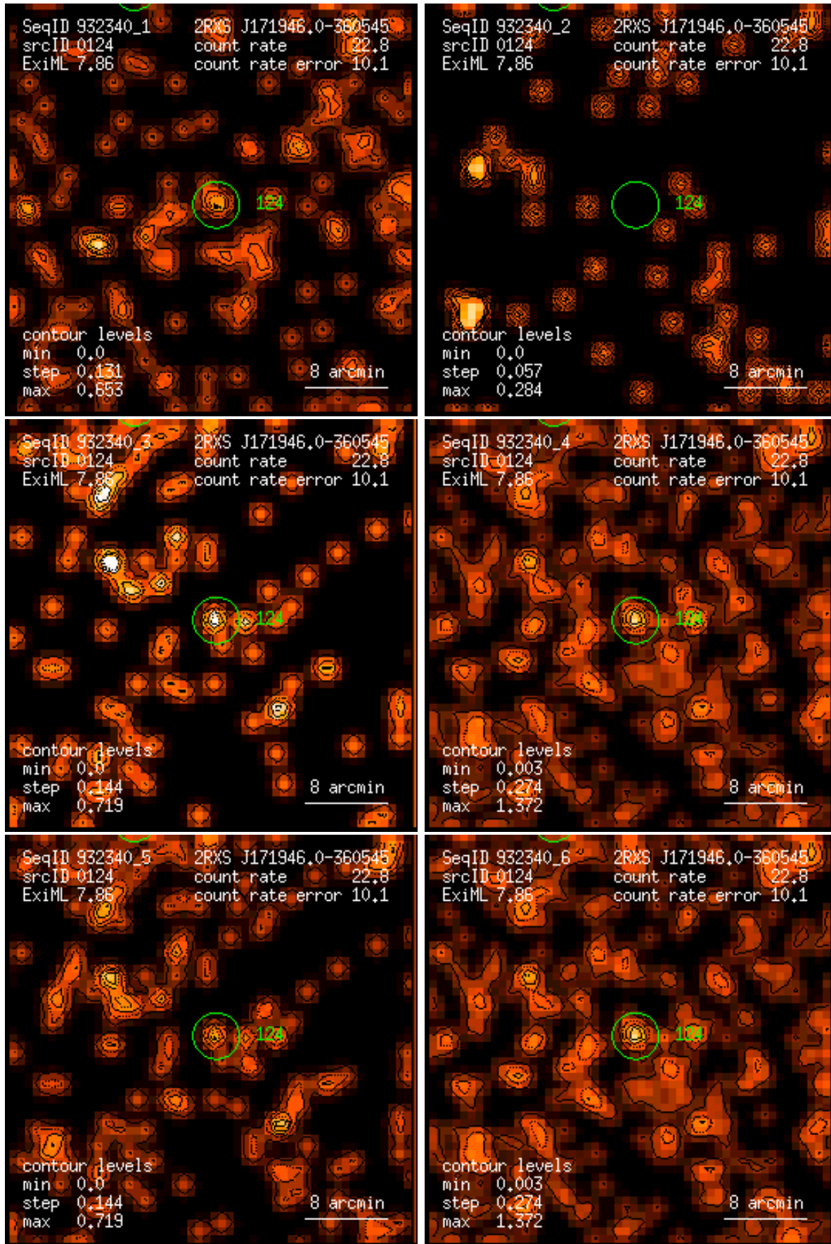
Figure 124: RASS 932340: detection 0124: band rate images, Gaussian filter: (1) PSPC channels 11 – 41, (2) 52 – 90, (3) 91 – 201, (4) 11 – 235, (5) 52 – 201, (6) 11 – 201. Broad band rates in counts/ks. Band rate contour levels in counts/ks/arcmin 2 .
