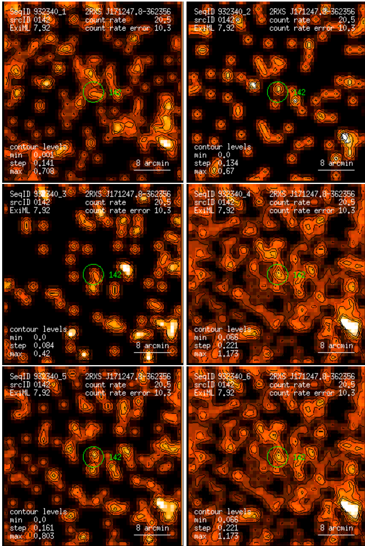
Figure 142: RASS 932340: detection 0142: band rate images, Gaussian filter: (1) PSPC channels 11 – 41, (2) 52 – 90, (3) 91 – 201, (4) 11 – 235, (5) 52 – 201, (6) 11 – 201. Broad band rates in counts/ks. Band rate contour levels in counts/ks/arcmin 2 .
