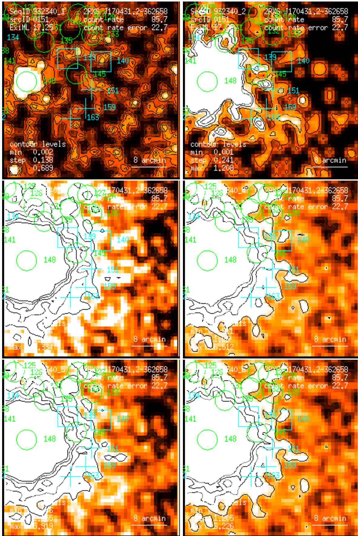
Figure 151: RASS 932340: detection 0151: band rate images, Gaussian filter: (1) PSPC channels 11 – 41, (2) 52 – 90, (3) 91 – 201, (4) 11 – 235, (5) 52 – 201, (6) 11 – 201. Broad band rates in counts/ks. Band rate contour levels in counts/ks/arcmin 2 .
