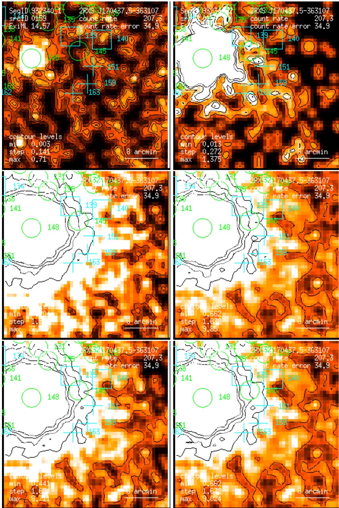
Figure 159: RASS 932340: detection 0159: band rate images, Gaussian filter: (1) PSPC channels 11 – 41, (2) 52 – 90, (3) 91 – 201, (4) 11 – 235, (5) 52 – 201, (6) 11 – 201. Broad band rates in counts/ks. Band rate contour levels in counts/ks/arcmin 2 .
