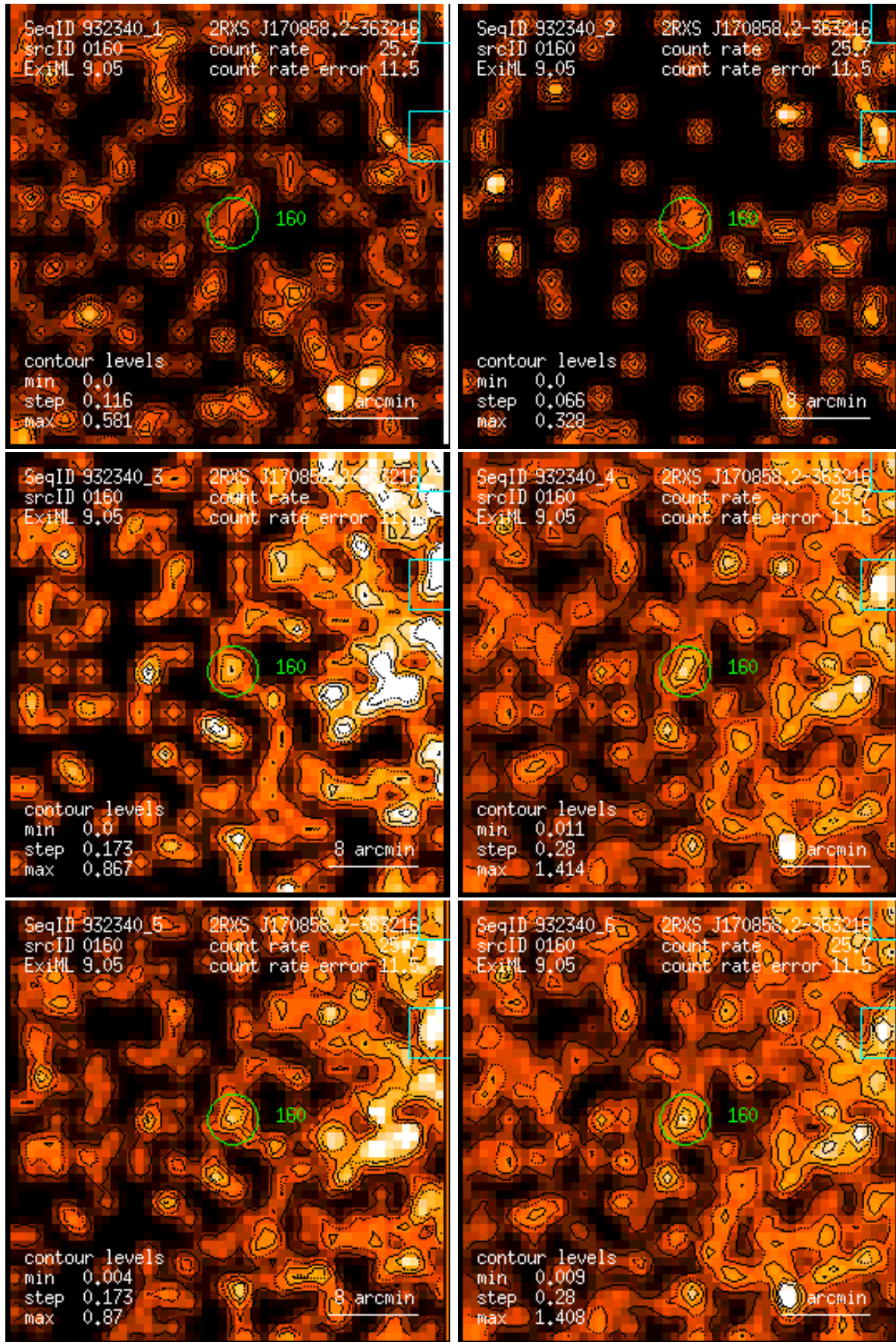
Figure 160: RASS 932340: detection 0160: band rate images, Gaussian filter: (1) PSPC channels 11 – 41, (2) 52 – 90, (3) 91 – 201, (4) 11 – 235, (5) 52 – 201, (6) 11 – 201. Broad band rates in counts/ks. Band rate contour levels in counts/ks/arcmin 2 .
