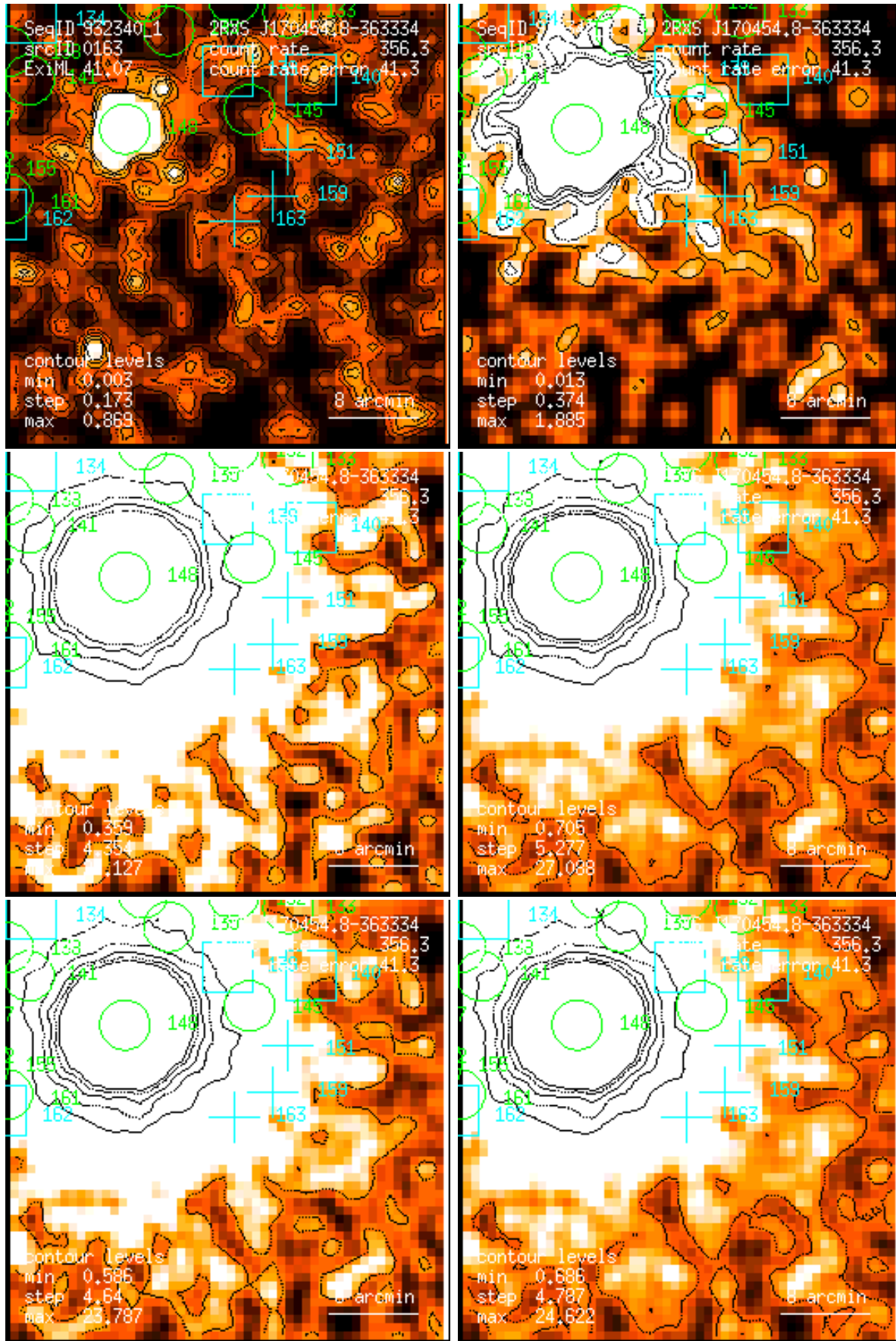
Figure 163: RASS 932340: detection 0163: band rate images, Gaussian filter: (1) PSPC channels 11 – 41, (2) 52 – 90, (3) 91 – 201, (4) 11 – 235, (5) 52 – 201, (6) 11 – 201. Broad band rates in counts/ks. Band rate contour levels in counts/ks/arcmin 2 .
