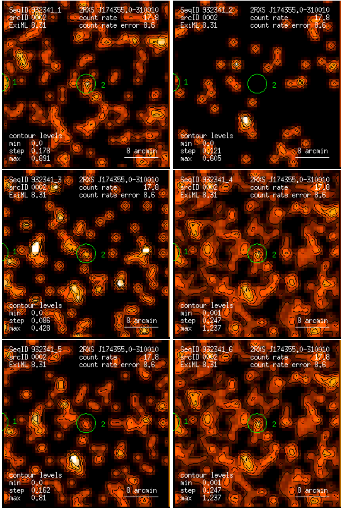
Figure 2: RASS 932341: detection 0002: band rate images, Gaussian filter: (1) PSPC channels 11 – 41, (2) 52 – 90, (3) 91 – 201, (4) 11 – 235, (5) 52 – 201, (6) 11 – 201. Broad band rates in counts/ks. Band rate contour levels in counts/ks/arcmin 2 .
