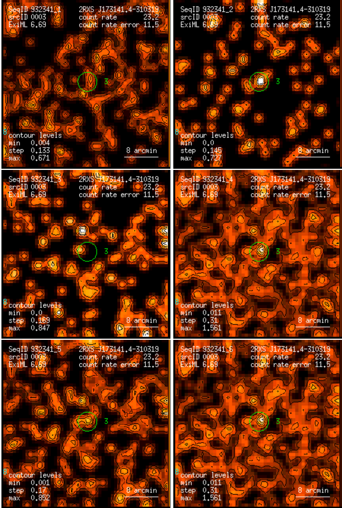
Figure 3: RASS 932341: detection 0003: band rate images, Gaussian filter: (1) PSPC channels 11 – 41, (2) 52 – 90, (3) 91 – 201, (4) 11 – 235, (5) 52 – 201, (6) 11 – 201. Broad band rates in counts/ks. Band rate contour levels in counts/ks/arcmin 2 .
