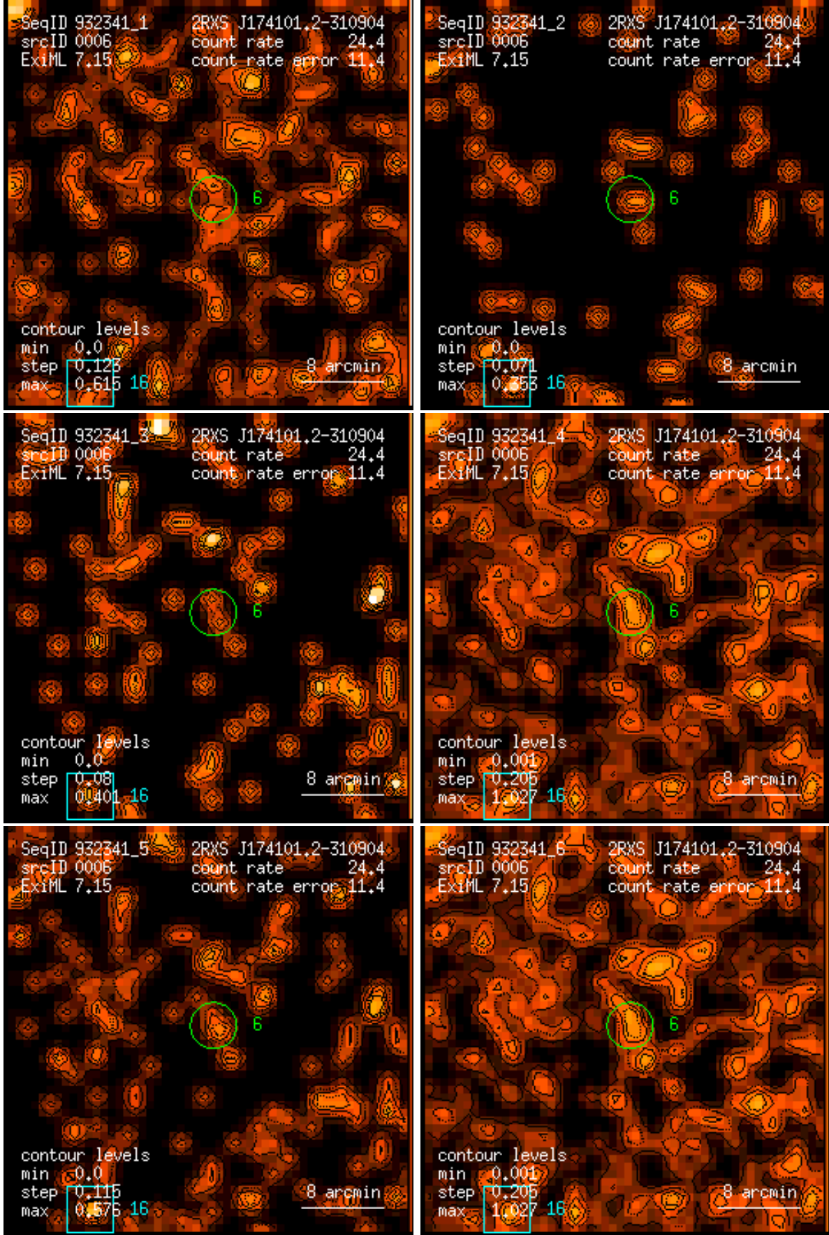
Figure 6: RASS 932341: detection 0006: band rate images, Gaussian filter: (1) PSPC channels 11 – 41, (2) 52 – 90, (3) 91 – 201, (4) 11 – 235, (5) 52 – 201, (6) 11 – 201. Broad band rates in counts/ks. Band rate contour levels in counts/ks/arcmin 2 .
