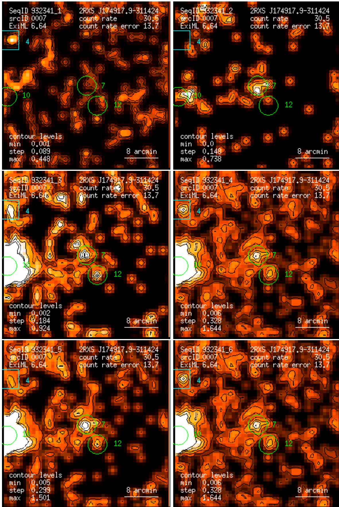
Figure 7: RASS 932341: detection 0007: band rate images, Gaussian filter: (1) PSPC channels 11 – 41, (2) 52 – 90, (3) 91 – 201, (4) 11 – 235, (5) 52 – 201, (6) 11 – 201. Broad band rates in counts/ks. Band rate contour levels in counts/ks/arcmin 2 .
