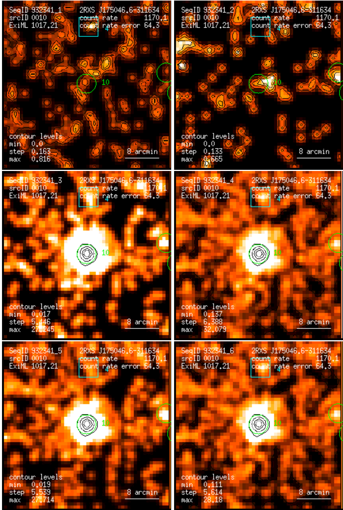
Figure 10: RASS 932341: detection 0010: band rate images, Gaussian filter: (1) PSPC channels 11 – 41, (2) 52 – 90, (3) 91 – 201, (4) 11 – 235, (5) 52 – 201, (6) 11 – 201. Broad band rates in counts/ks. Band rate contour levels in counts/ks/arcmin 2 .
