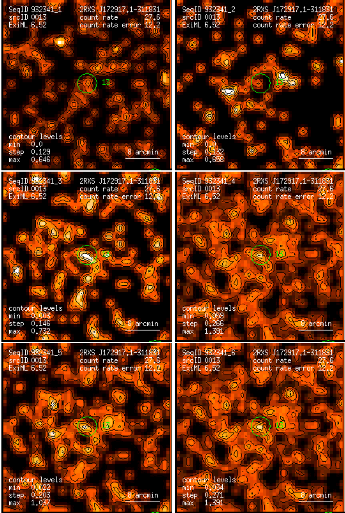
Figure 13: RASS 932341: detection 0013: band rate images, Gaussian filter: (1) PSPC channels 11 – 41, (2) 52 – 90, (3) 91 – 201, (4) 11 – 235, (5) 52 – 201, (6) 11 – 201. Broad band rates in counts/ks. Band rate contour levels in counts/ks/arcmin 2 .
