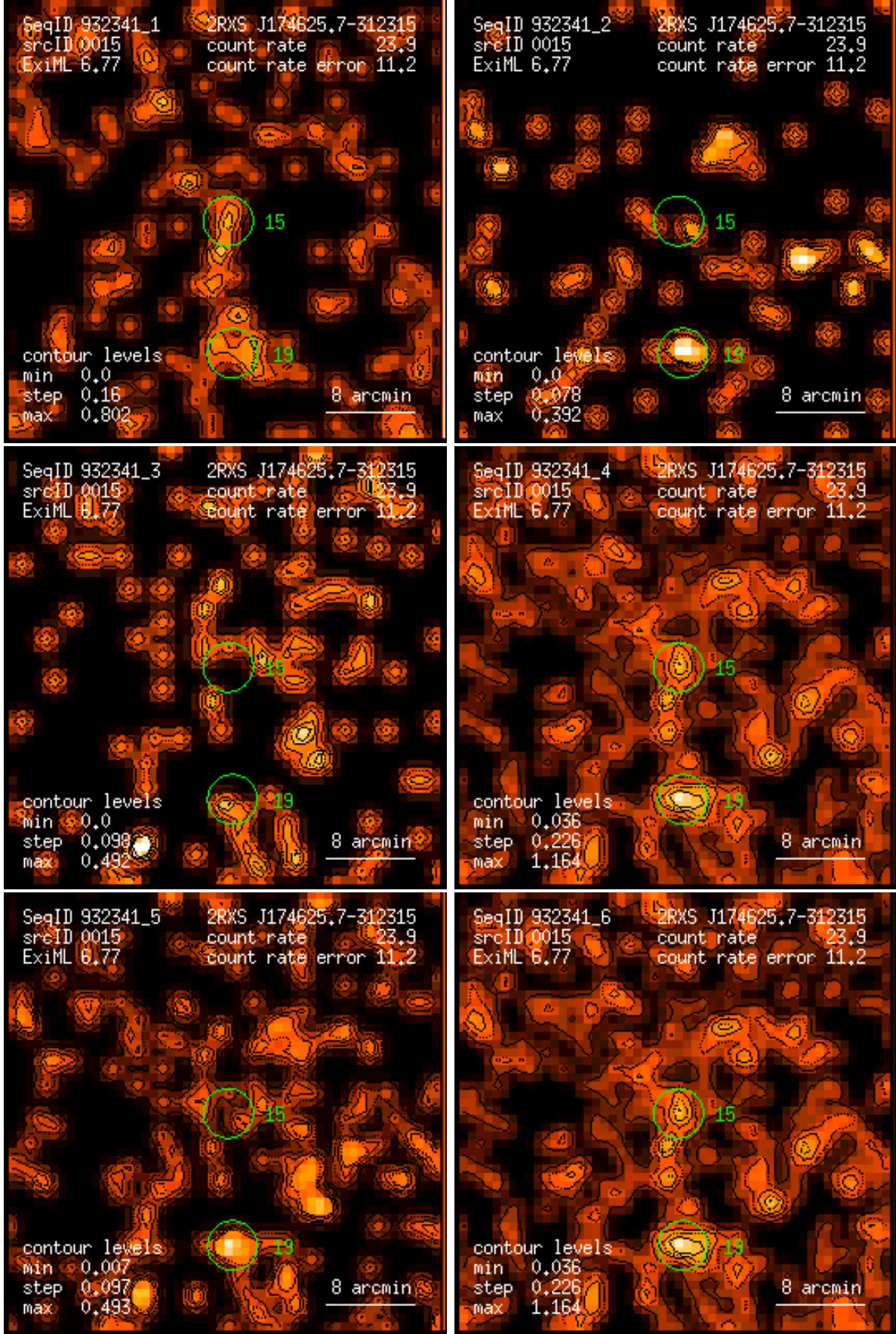
Figure 15: RASS 932341: detection 0015: band rate images, Gaussian filter: (1) PSPC channels 11 – 41, (2) 52 – 90, (3) 91 – 201, (4) 11 – 235, (5) 52 – 201, (6) 11 – 201. Broad band rates in counts/ks. Band rate contour levels in counts/ks/arcmin 2 .
