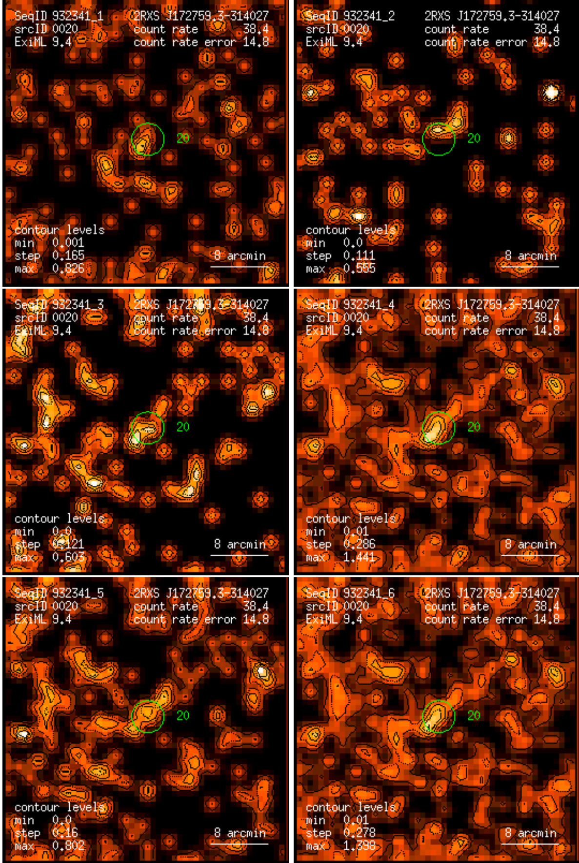
Figure 20: RASS 932341: detection 0020: band rate images, Gaussian filter: (1) PSPC channels 11 – 41, (2) 52 – 90, (3) 91 – 201, (4) 11 – 235, (5) 52 – 201, (6) 11 – 201. Broad band rates in counts/ks. Band rate contour levels in counts/ks/arcmin 2 .
