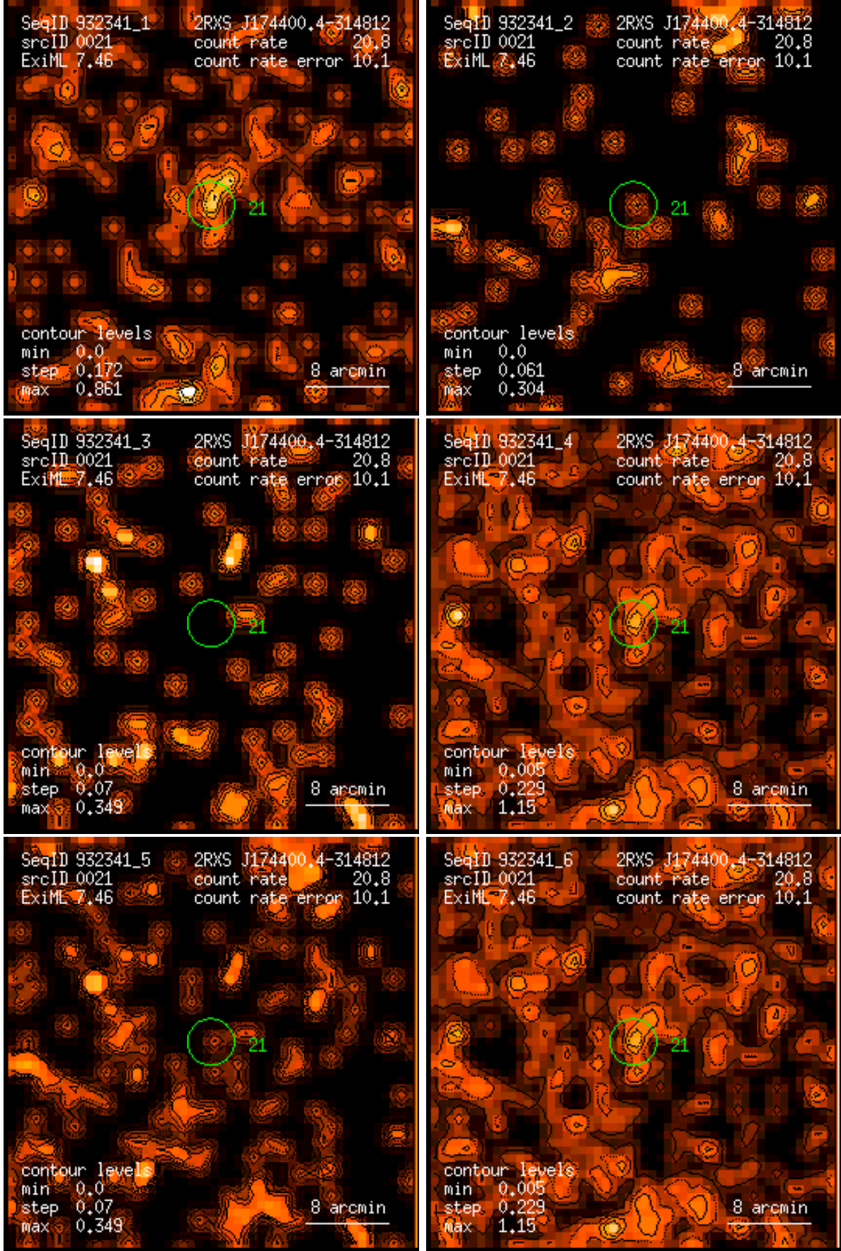
Figure 21: RASS 932341: detection 0021: band rate images, Gaussian filter: (1) PSPC channels 11 – 41, (2) 52 – 90, (3) 91 – 201, (4) 11 – 235, (5) 52 – 201, (6) 11 – 201. Broad band rates in counts/ks. Band rate contour levels in counts/ks/arcmin 2 .
