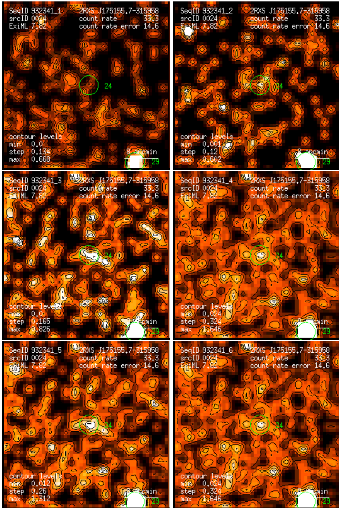
Figure 24: RASS 932341: detection 0024: band rate images, Gaussian filter: (1) PSPC channels 11 – 41, (2) 52 – 90, (3) 91 – 201, (4) 11 – 235, (5) 52 – 201, (6) 11 – 201. Broad band rates in counts/ks. Band rate contour levels in counts/ks/arcmin 2 .
