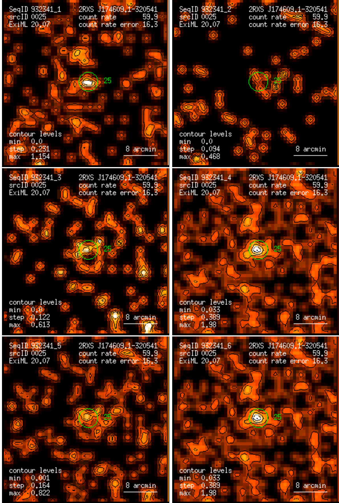
Figure 25: RASS 932341: detection 0025: band rate images, Gaussian filter: (1) PSPC channels 11 – 41, (2) 52 – 90, (3) 91 – 201, (4) 11 – 235, (5) 52 – 201, (6) 11 – 201. Broad band rates in counts/ks. Band rate contour levels in counts/ks/arcmin 2 .
