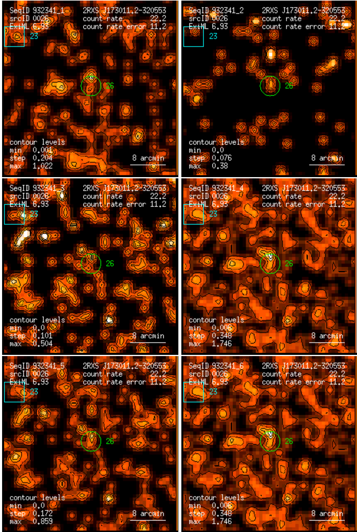
Figure 26: RASS 932341: detection 0026: band rate images, Gaussian filter: (1) PSPC channels 11 – 41, (2) 52 – 90, (3) 91 – 201, (4) 11 – 235, (5) 52 – 201, (6) 11 – 201. Broad band rates in counts/ks. Band rate contour levels in counts/ks/arcmin 2 .
