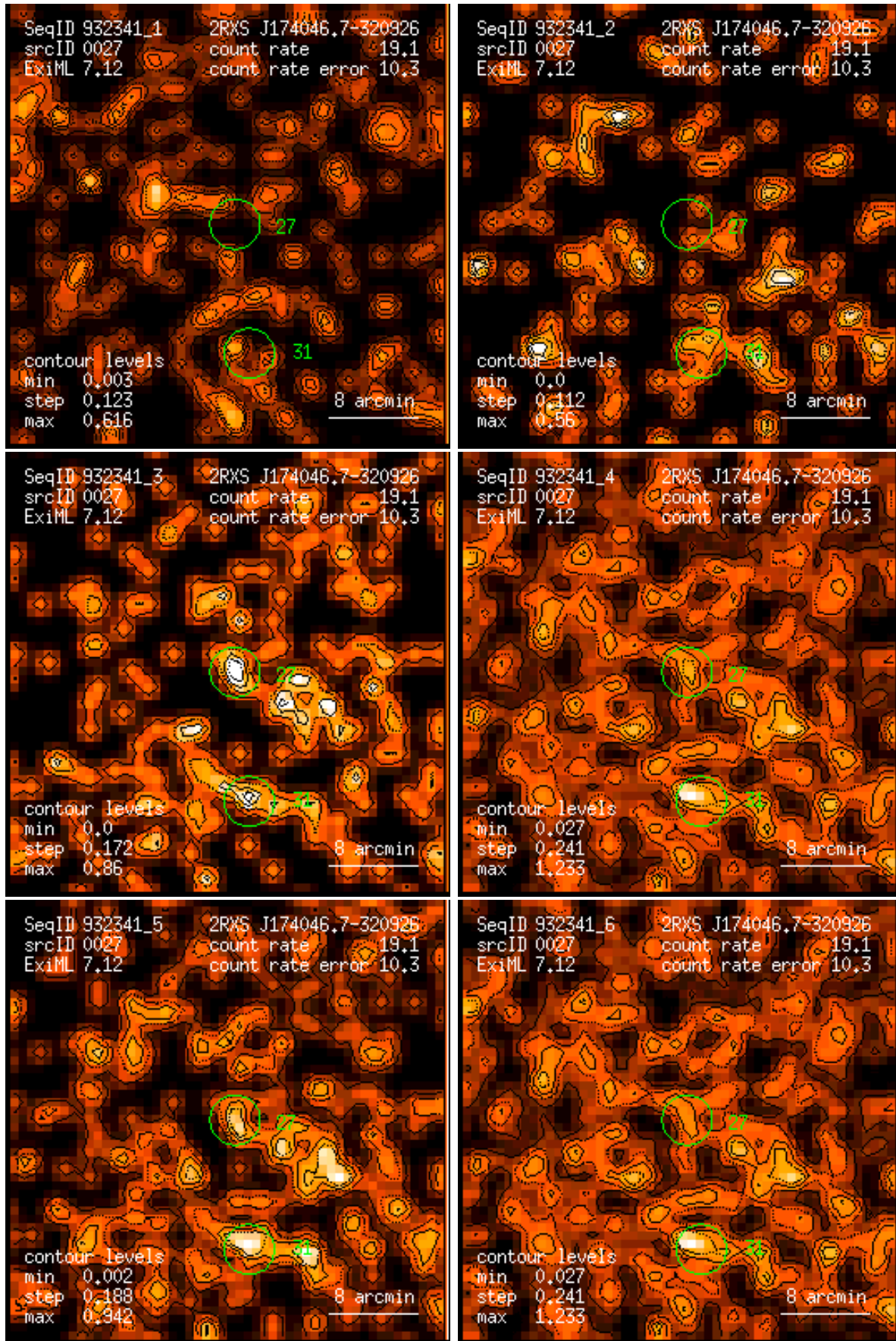
Figure 27: RASS 932341: detection 0027: band rate images, Gaussian filter: (1) PSPC channels 11 – 41, (2) 52 – 90, (3) 91 – 201, (4) 11 – 235, (5) 52 – 201, (6) 11 – 201. Broad band rates in counts/ks. Band rate contour levels in counts/ks/arcmin 2 .
