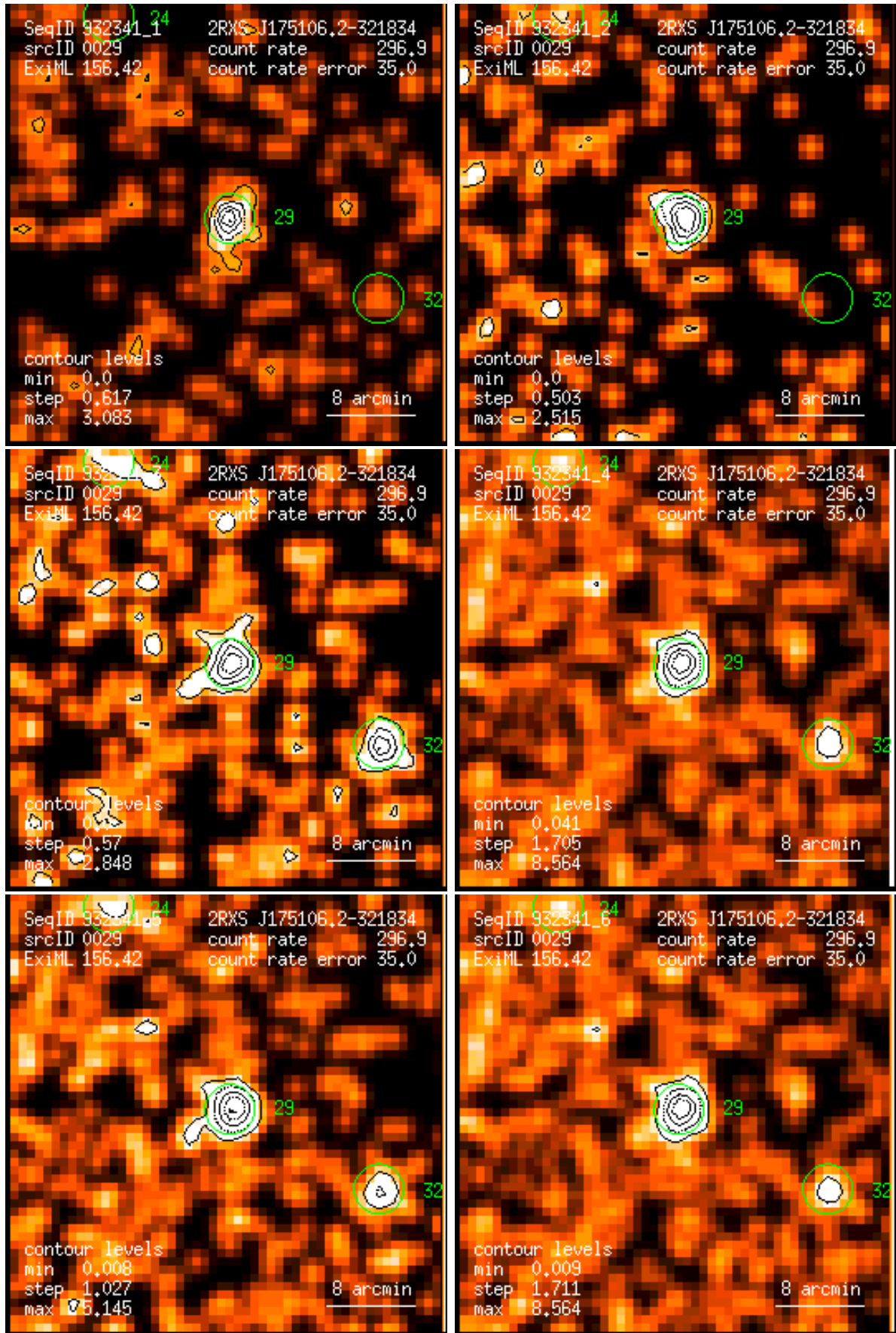
Figure 29: RASS 932341: detection 0029: band rate images, Gaussian filter: (1) PSPC channels 11 – 41, (2) 52 – 90, (3) 91 – 201, (4) 11 – 235, (5) 52 – 201, (6) 11 – 201. Broad band rates in counts/ks. Band rate contour levels in counts/ks/arcmin 2 .
