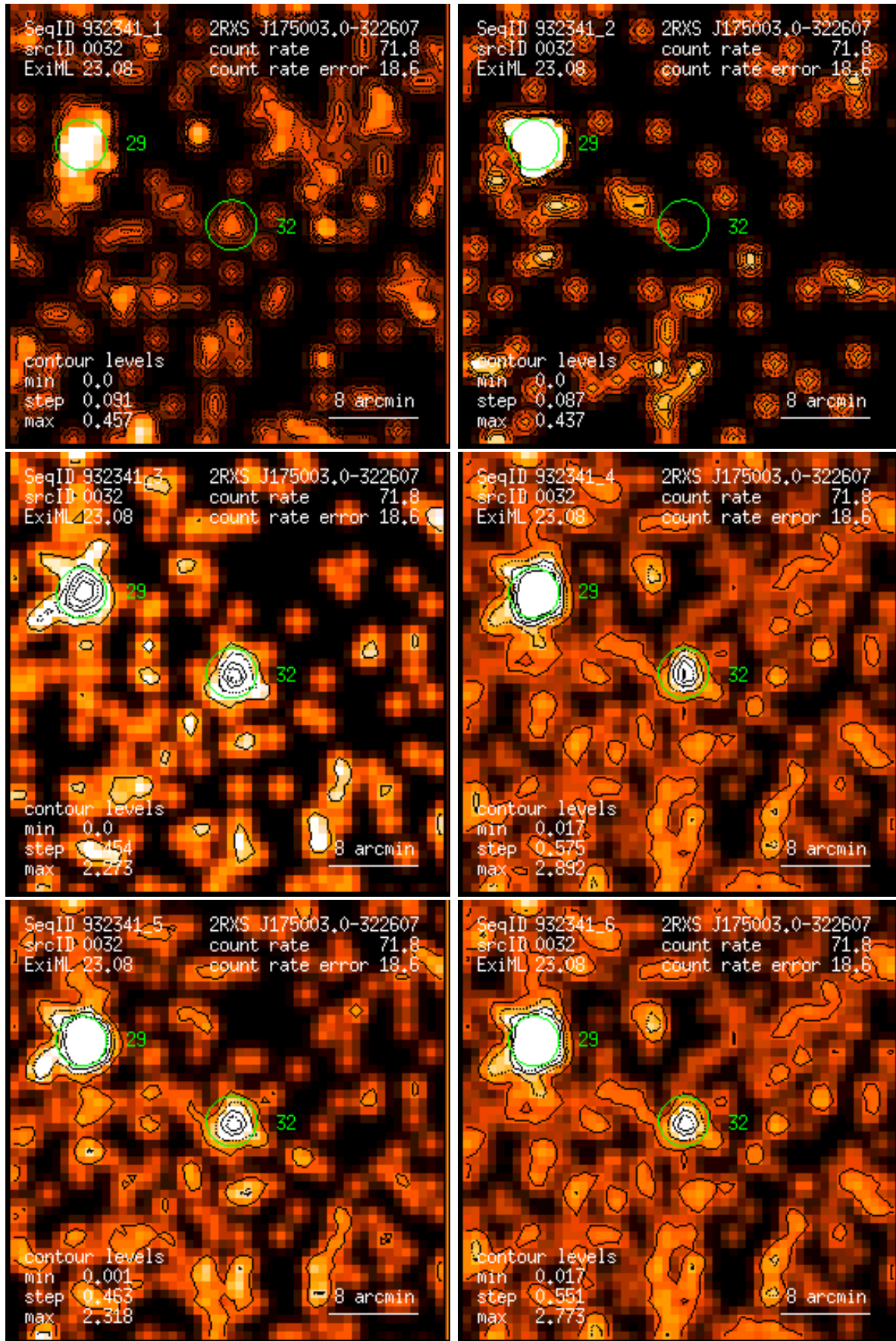
Figure 32: RASS 932341: detection 0032: band rate images, Gaussian filter: (1) PSPC channels 11 – 41, (2) 52 – 90, (3) 91 – 201, (4) 11 – 235, (5) 52 – 201, (6) 11 – 201. Broad band rates in counts/ks. Band rate contour levels in counts/ks/arcmin 2 .
