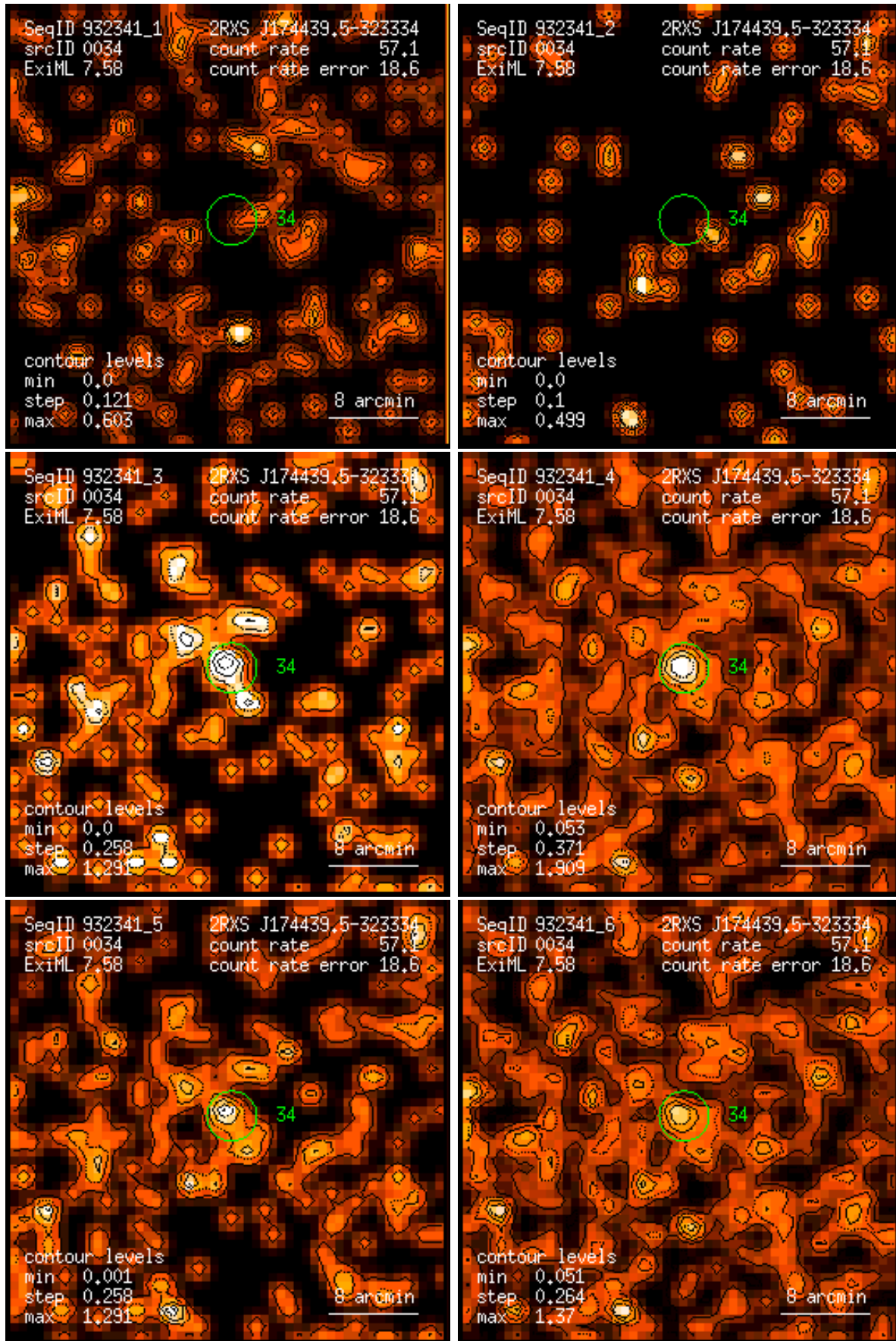
Figure 34: RASS 932341: detection 0034: band rate images, Gaussian filter: (1) PSPC channels 11 – 41, (2) 52 – 90, (3) 91 – 201, (4) 11 – 235, (5) 52 – 201, (6) 11 – 201. Broad band rates in counts/ks. Band rate contour levels in counts/ks/arcmin 2 .
