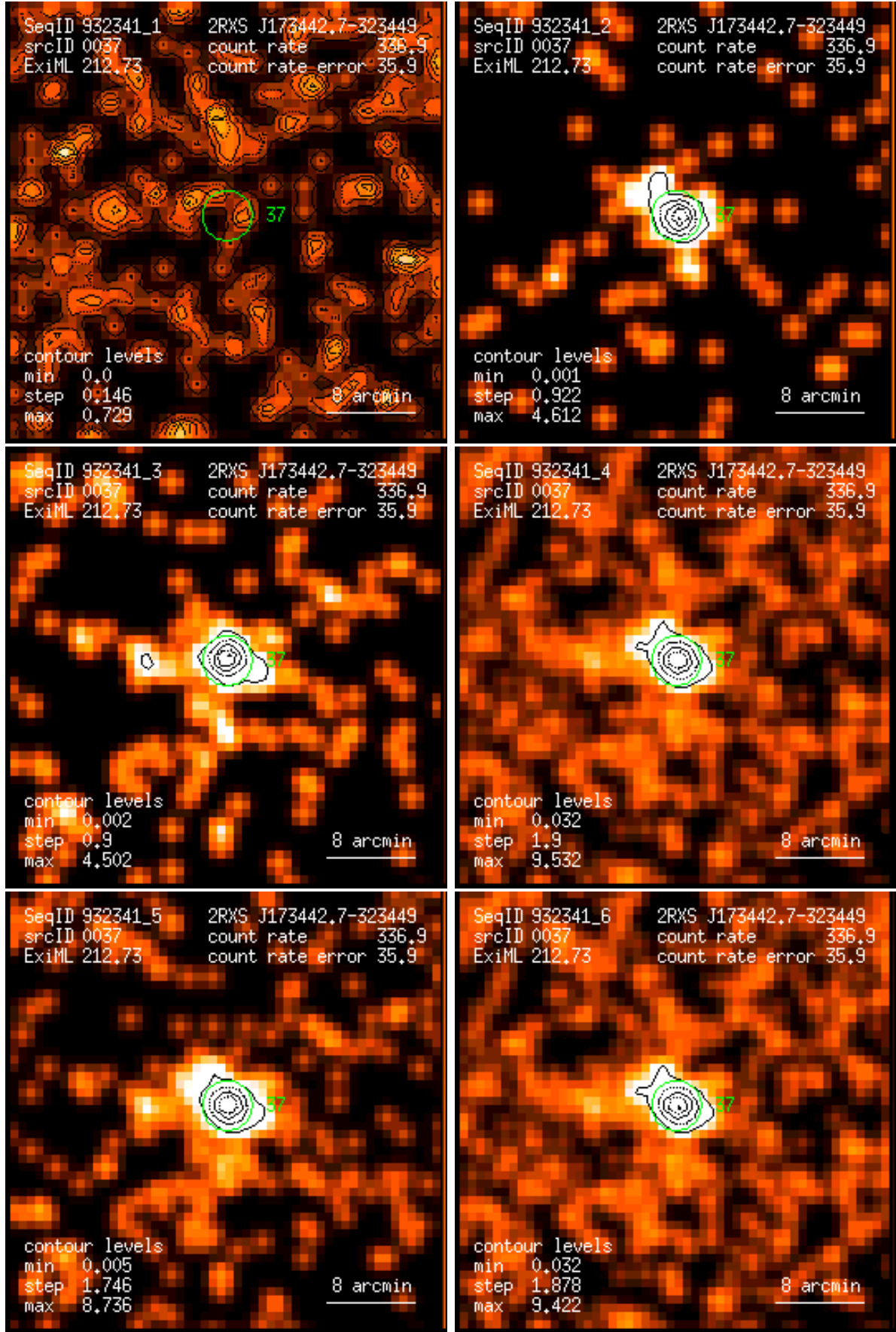
Figure 37: RASS 932341: detection 0037: band rate images, Gaussian filter: (1) PSPC channels 11 – 41, (2) 52 – 90, (3) 91 – 201, (4) 11 – 235, (5) 52 – 201, (6) 11 – 201. Broad band rates in counts/ks. Band rate contour levels in counts/ks/arcmin 2 .
