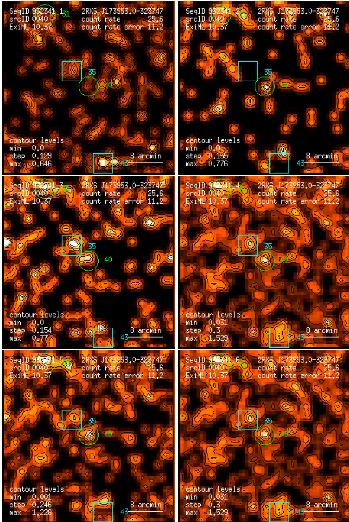
Figure 40: RASS 932341: detection 0040: band rate images, Gaussian filter: (1) PSPC channels 11 – 41, (2) 52 – 90, (3) 91 – 201, (4) 11 – 235, (5) 52 – 201, (6) 11 – 201. Broad band rates in counts/ks. Band rate contour levels in counts/ks/arcmin 2 .
