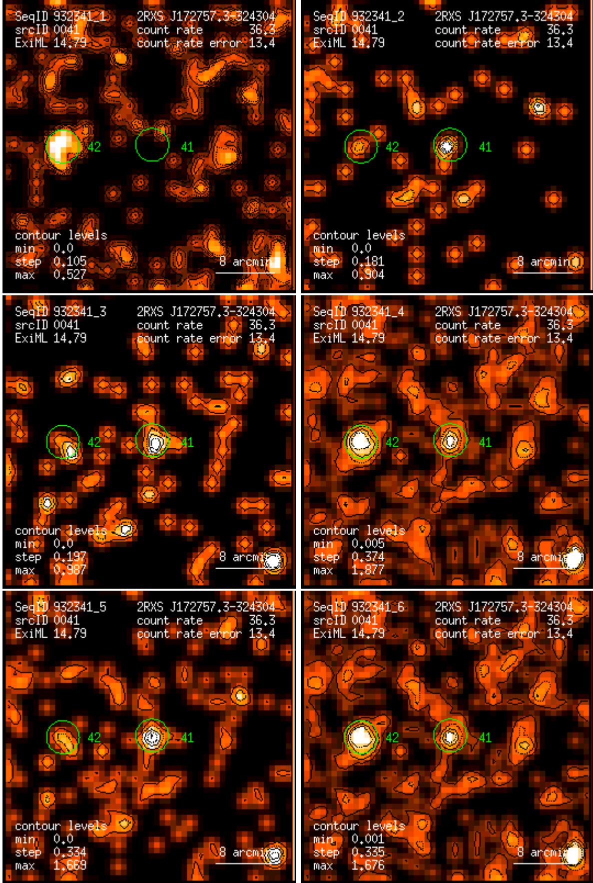
Figure 41: RASS 932341: detection 0041: band rate images, Gaussian filter: (1) PSPC channels 11 – 41, (2) 52 – 90, (3) 91 – 201, (4) 11 – 235, (5) 52 – 201, (6) 11 – 201. Broad band rates in counts/ks. Band rate contour levels in counts/ks/arcmin 2 .
