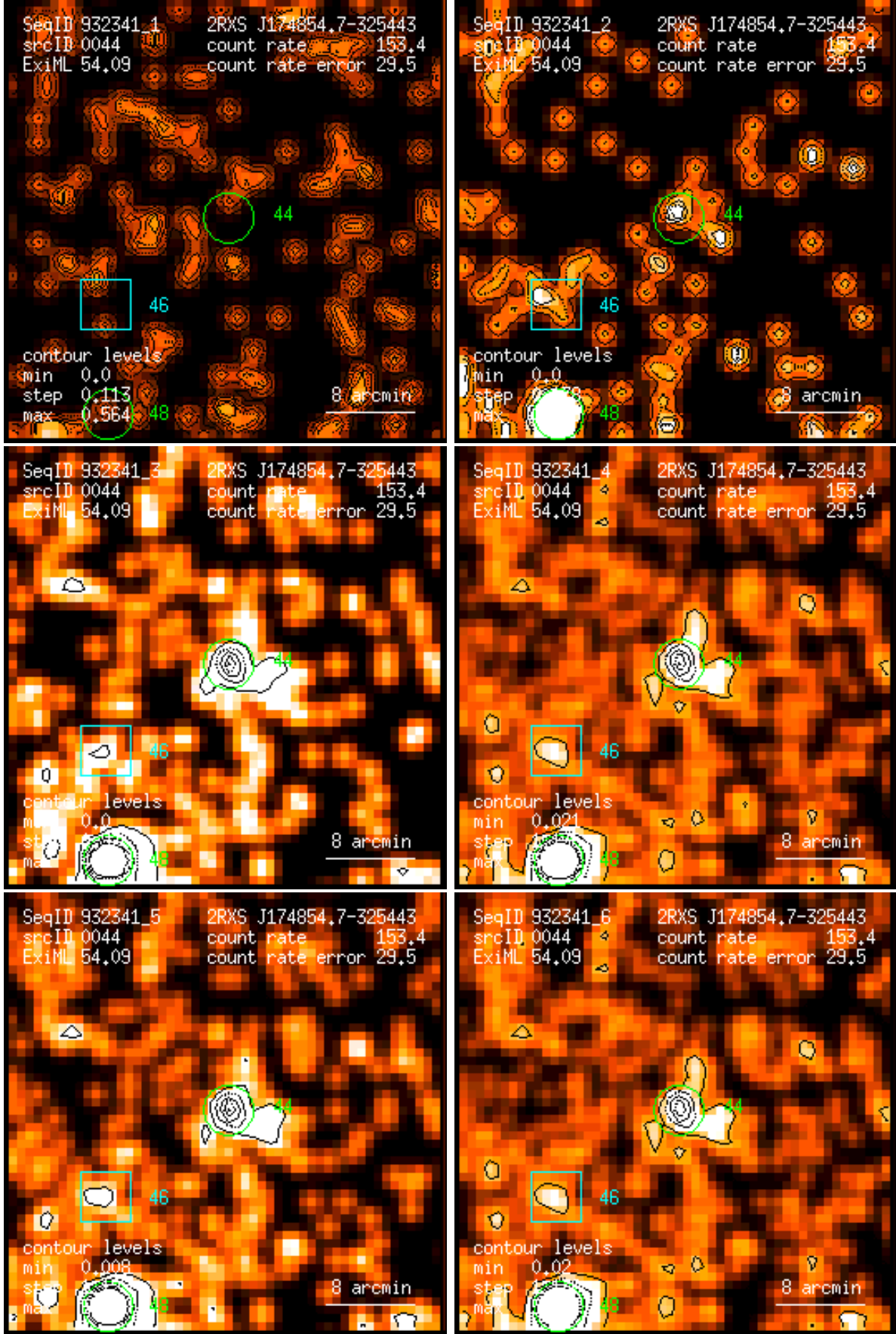
Figure 44: RASS 932341: detection 0044: band rate images, Gaussian filter: (1) PSPC channels 11 – 41, (2) 52 – 90, (3) 91 – 201, (4) 11 – 235, (5) 52 – 201, (6) 11 – 201. Broad band rates in counts/ks. Band rate contour levels in counts/ks/arcmin 2 .
