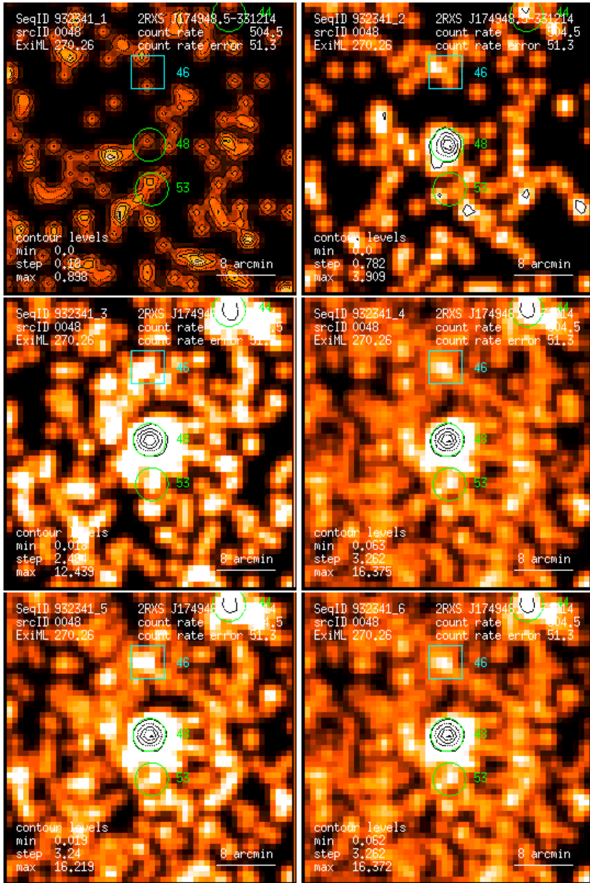
Figure 48: RASS 932341: detection 0048: band rate images, Gaussian filter: (1) PSPC channels 11 – 41, (2) 52 – 90, (3) 91 – 201, (4) 11 – 235, (5) 52 – 201, (6) 11 – 201. Broad band rates in counts/ks. Band rate contour levels in counts/ks/arcmin 2 .
