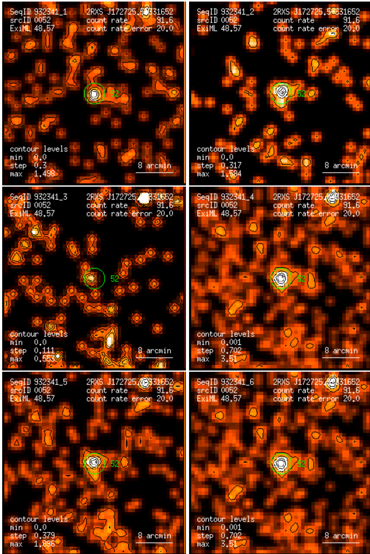
Figure 52: RASS 932341: detection 0052: band rate images, Gaussian filter: (1) PSPC channels 11 – 41, (2) 52 – 90, (3) 91 – 201, (4) 11 – 235, (5) 52 – 201, (6) 11 – 201. Broad band rates in counts/ks. Band rate contour levels in counts/ks/arcmin 2 .
