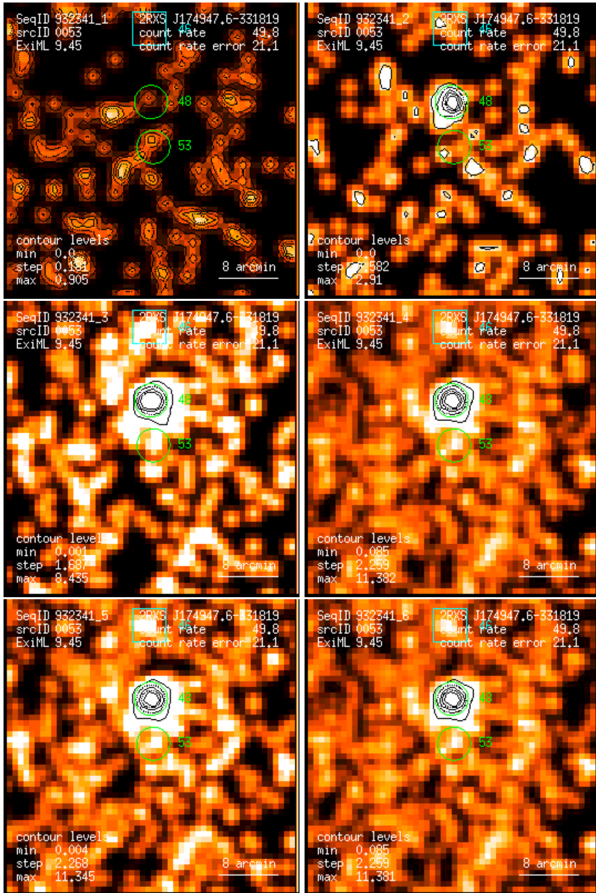
Figure 53: RASS 932341: detection 0053: band rate images, Gaussian filter: (1) PSPC channels 11 – 41, (2) 52 – 90, (3) 91 – 201, (4) 11 – 235, (5) 52 – 201, (6) 11 – 201. Broad band rates in counts/ks. Band rate contour levels in counts/ks/arcmin 2 .
