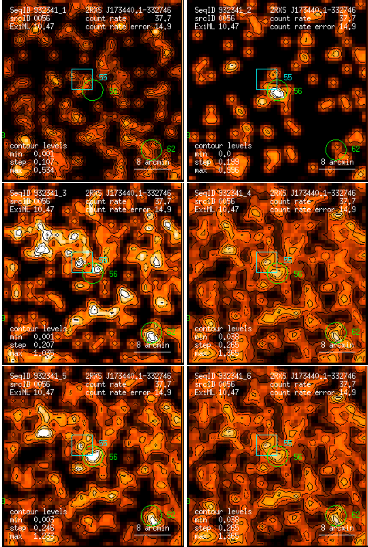
Figure 56: RASS 932341: detection 0056: band rate images, Gaussian filter: (1) PSPC channels 11 – 41, (2) 52 – 90, (3) 91 – 201, (4) 11 – 235, (5) 52 – 201, (6) 11 – 201. Broad band rates in counts/ks. Band rate contour levels in counts/ks/arcmin 2 .
