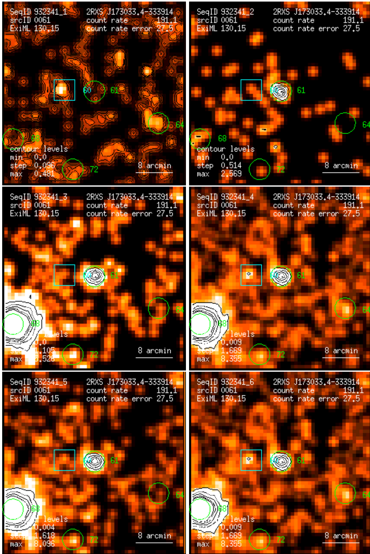
Figure 61: RASS 932341: detection 0061: band rate images, Gaussian filter: (1) PSPC channels 11 – 41, (2) 52 – 90, (3) 91 – 201, (4) 11 – 235, (5) 52 – 201, (6) 11 – 201. Broad band rates in counts/ks. Band rate contour levels in counts/ks/arcmin 2 .
