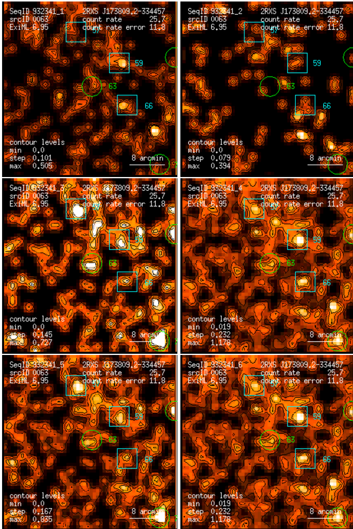
Figure 63: RASS 932341: detection 0063: band rate images, Gaussian filter: (1) PSPC channels 11 – 41, (2) 52 – 90, (3) 91 – 201, (4) 11 – 235, (5) 52 – 201, (6) 11 – 201. Broad band rates in counts/ks. Band rate contour levels in counts/ks/arcmin 2 .
