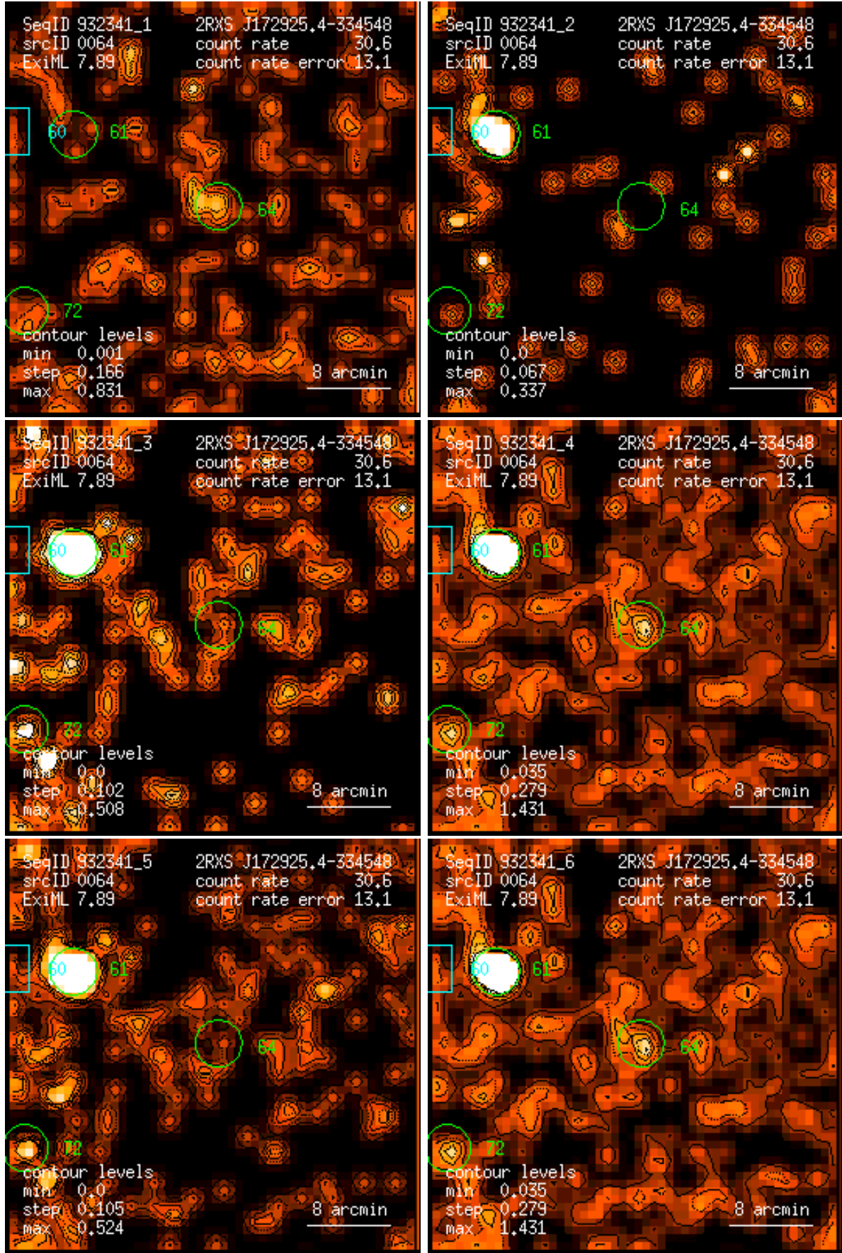
Figure 64: RASS 932341: detection 0064: band rate images, Gaussian filter: (1) PSPC channels 11 – 41, (2) 52 – 90, (3) 91 – 201, (4) 11 – 235, (5) 52 – 201, (6) 11 – 201. Broad band rates in counts/ks. Band rate contour levels in counts/ks/arcmin 2 .
