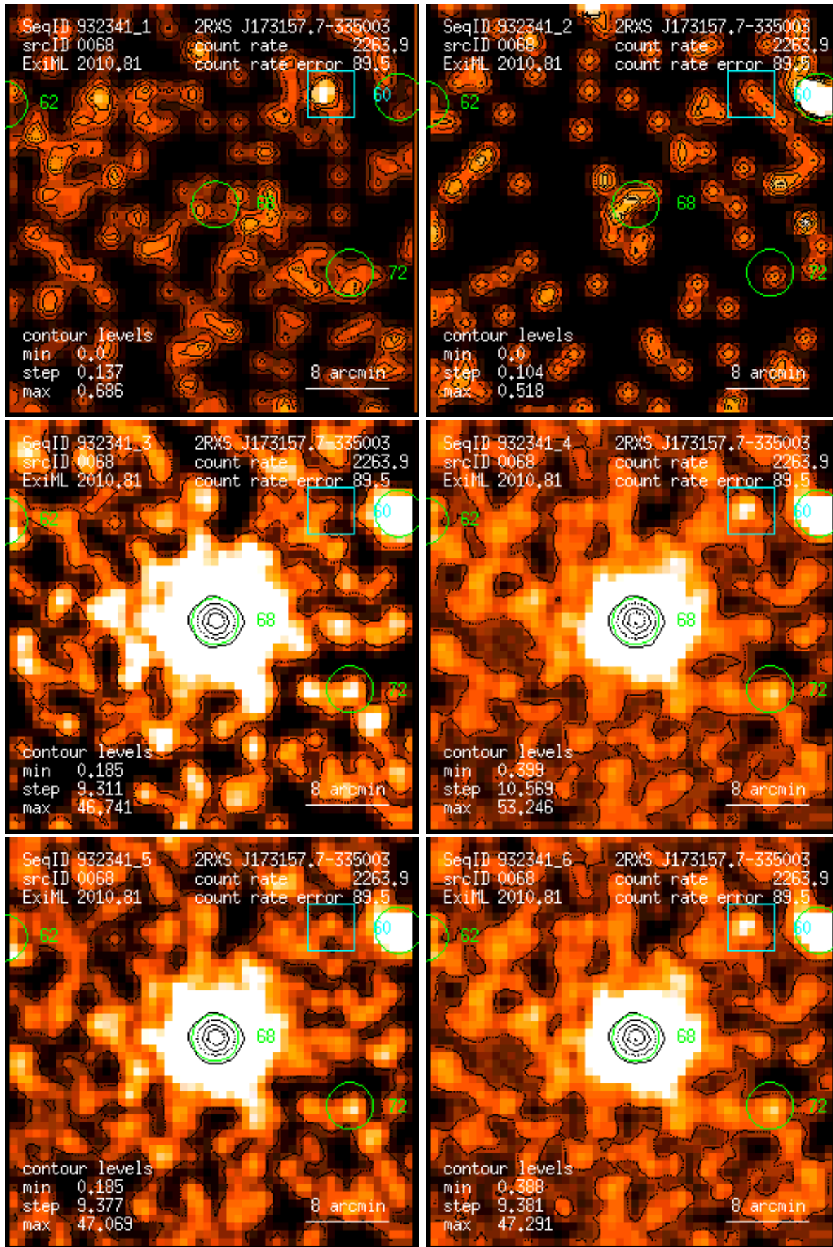
Figure 68: RASS 932341: detection 0068: band rate images, Gaussian filter: (1) PSPC channels 11 – 41, (2) 52 – 90, (3) 91 – 201, (4) 11 – 235, (5) 52 – 201, (6) 11 – 201. Broad band rates in counts/ks. Band rate contour levels in counts/ks/arcmin 2 .
