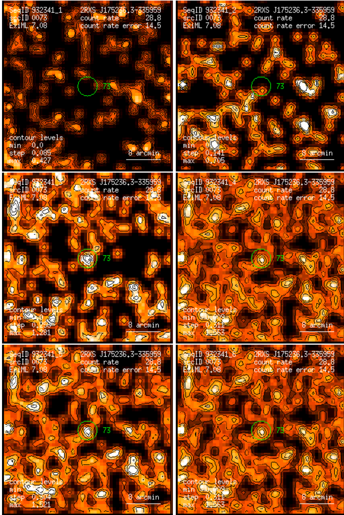
Figure 73: RASS 932341: detection 0073: band rate images, Gaussian filter: (1) PSPC channels 11 – 41, (2) 52 – 90, (3) 91 – 201, (4) 11 – 235, (5) 52 – 201, (6) 11 – 201. Broad band rates in counts/ks. Band rate contour levels in counts/ks/arcmin 2 .
