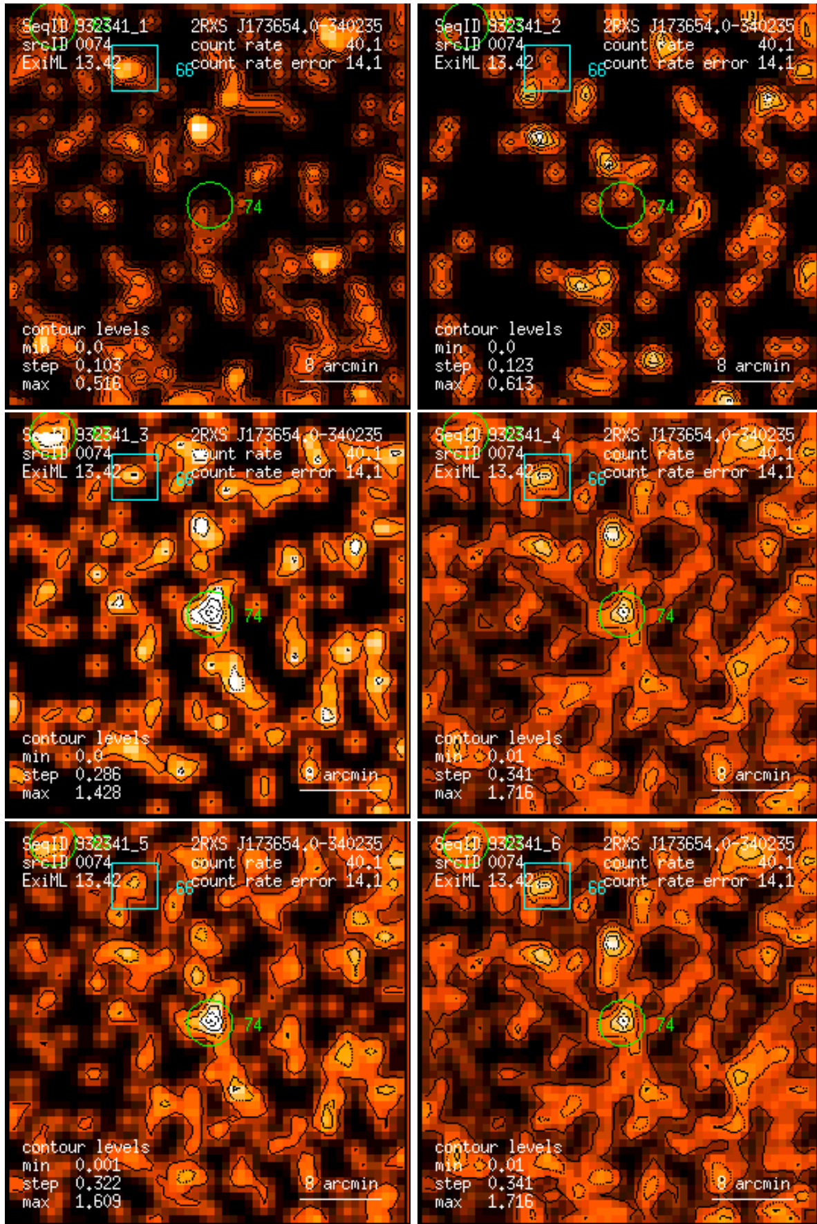
Figure 74: RASS 932341: detection 0074: band rate images, Gaussian filter: (1) PSPC channels 11 – 41, (2) 52 – 90, (3) 91 – 201, (4) 11 – 235, (5) 52 – 201, (6) 11 – 201. Broad band rates in counts/ks. Band rate contour levels in counts/ks/arcmin 2 .
