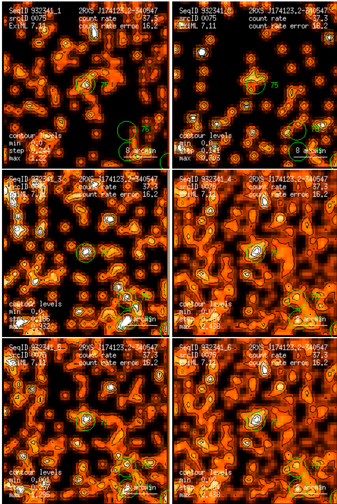
Figure 75: RASS 932341: detection 0075: band rate images, Gaussian filter: (1) PSPC channels 11 – 41, (2) 52 – 90, (3) 91 – 201, (4) 11 – 235, (5) 52 – 201, (6) 11 – 201. Broad band rates in counts/ks. Band rate contour levels in counts/ks/arcmin 2 .
