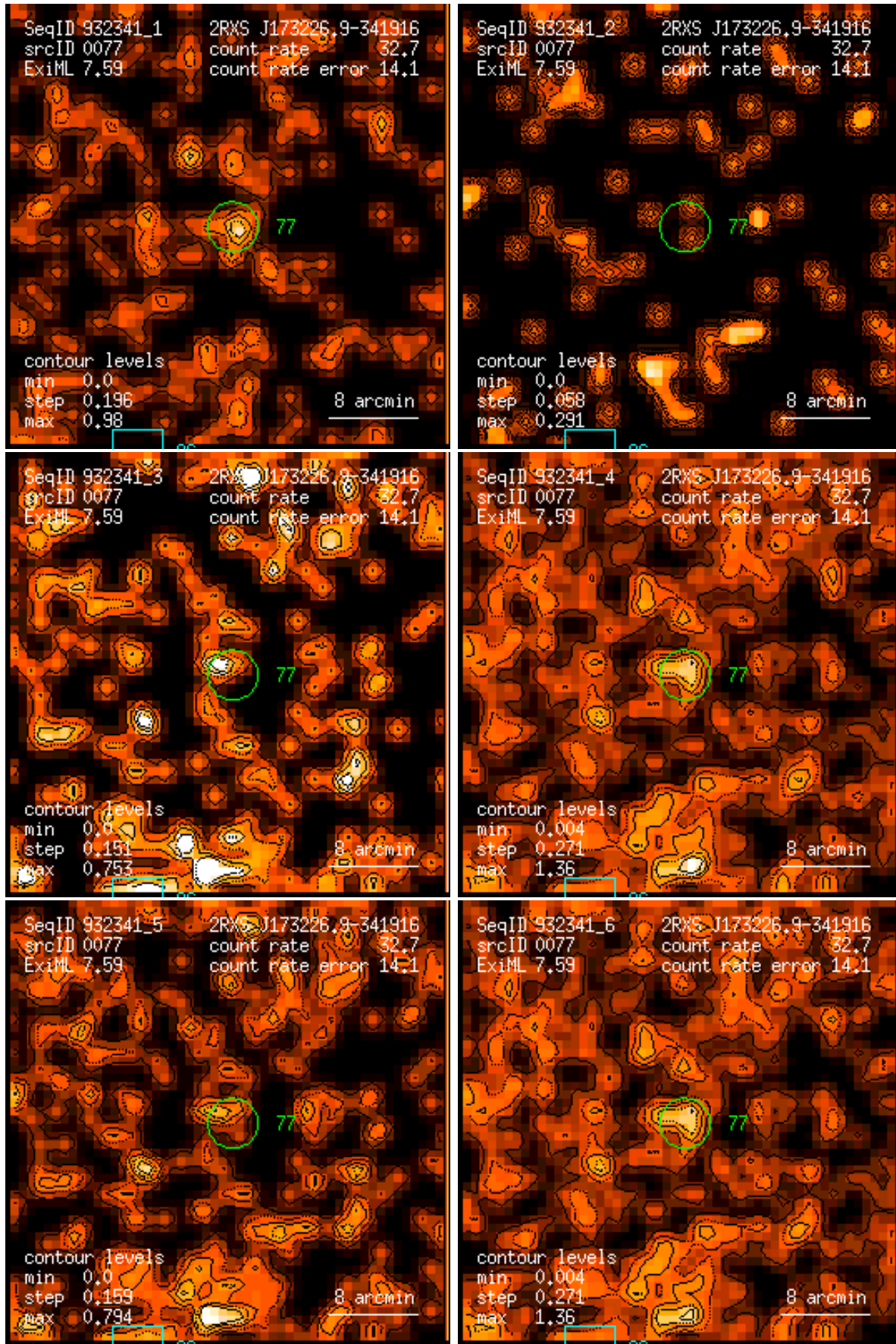
Figure 77: RASS 932341: detection 0077: band rate images, Gaussian filter: (1) PSPC channels 11 – 41, (2) 52 – 90, (3) 91 – 201, (4) 11 – 235, (5) 52 – 201, (6) 11 – 201. Broad band rates in counts/ks. Band rate contour levels in counts/ks/arcmin 2 .
